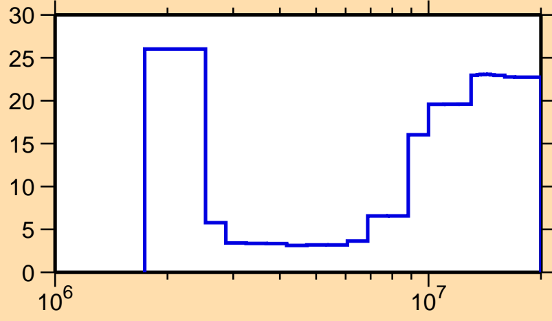
\Delta\sigma/\sigma vs. E for ^{58}\text{Mn}(n,n\text{cont.})
