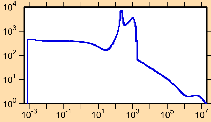
\sigma vs. E for ^{58}\text{Mn}(n,\text{el.})
