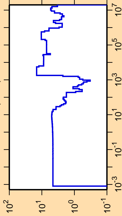
\Delta\sigma/\sigma vs. E for ^{58}\text{Mn}(n,\text{el.})
