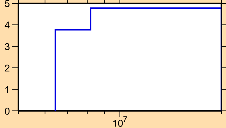
\Delta\sigma/\sigma vs. E for ^{58}\text{Mn}(n,\text{el.})
