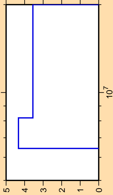
\Delta\sigma/\sigma vs. E for ^{58}\text{Mn}(n,2n)
