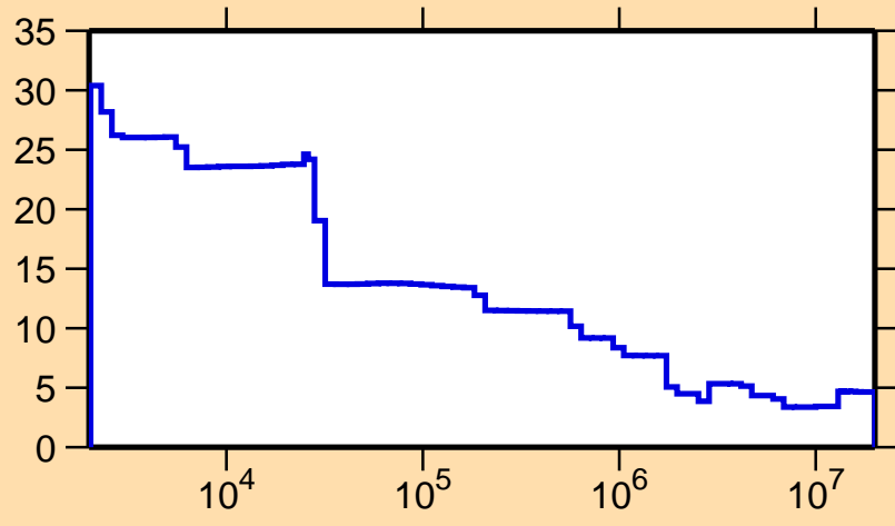
\Delta\sigma/\sigma vs. E for ^{60}\text{Mn}(n,\text{nonel.})
