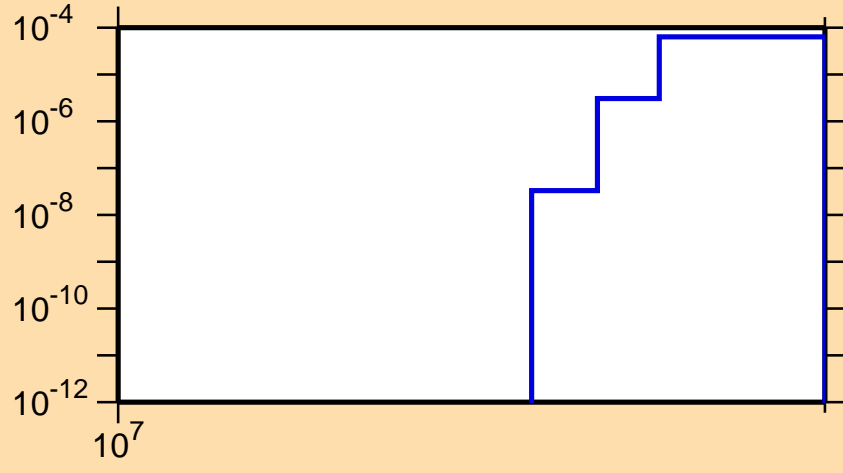
\sigma vs. E for ^{60}\text{Mn}(n,\text{nd})
