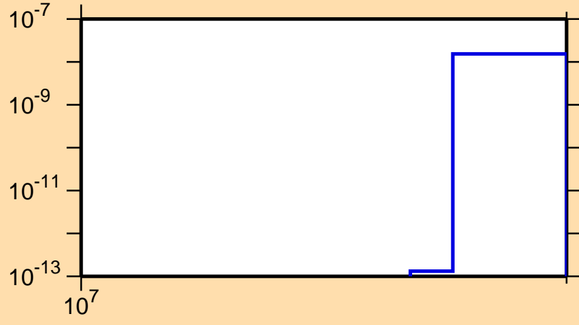
\sigma vs. E for ^{60}\text{Mn}(n,2n\alpha)
