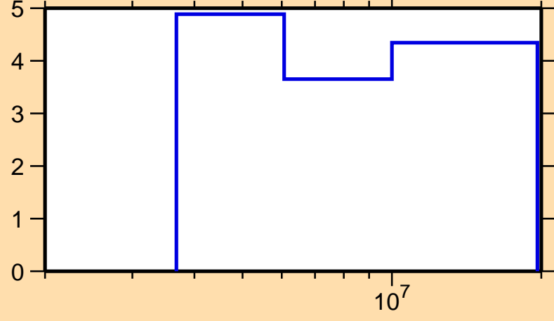
\Delta\sigma/\sigma vs. E for ^{60}\text{Mn}(n,\text{nonel.})
