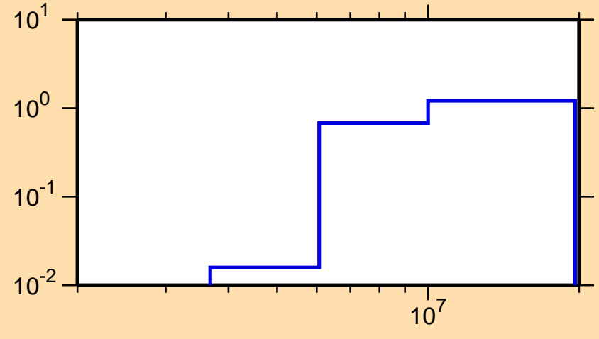
\sigma vs. E for ^{60}\text{Mn}(n,2n)
