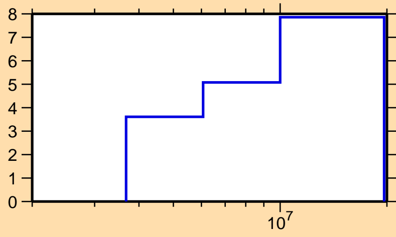
\Delta\sigma/\sigma vs. E for ^{60}\text{Mn}(n,el.)
