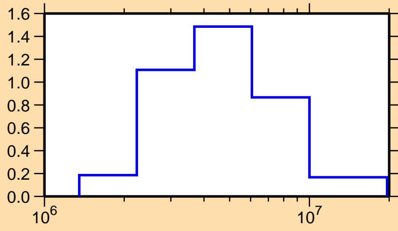
\sigma vs. E for ^{60}\text{Mn}(n,n\text{cont.})
