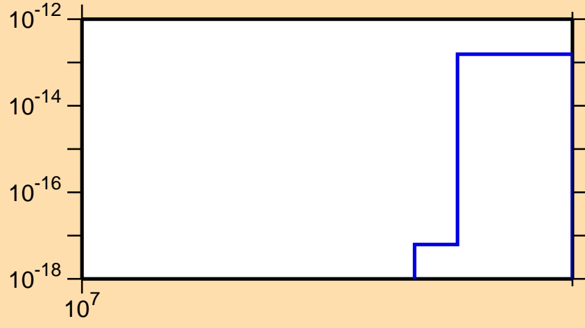
\sigma vs. E for ^{85}\text{Mo}(n,2n\alpha)
