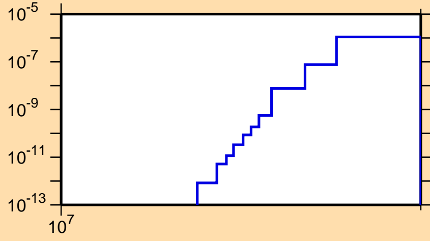
\sigma vs. E for ^{85}\text{Mo} (mt 45)
