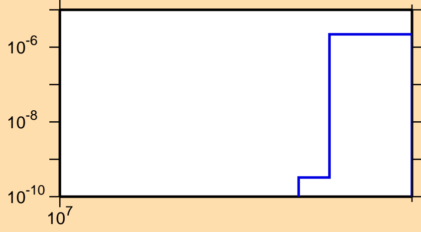
\sigma vs. E for ^{85}\text{Mo}(n,2np)
