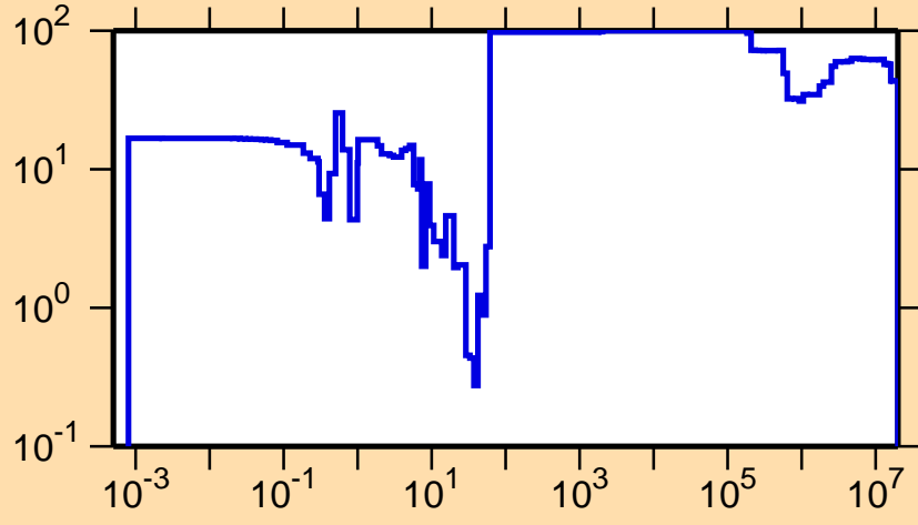
\Delta\sigma/\sigma vs. E for ^{85}\text{Mo}(n,\gamma)
