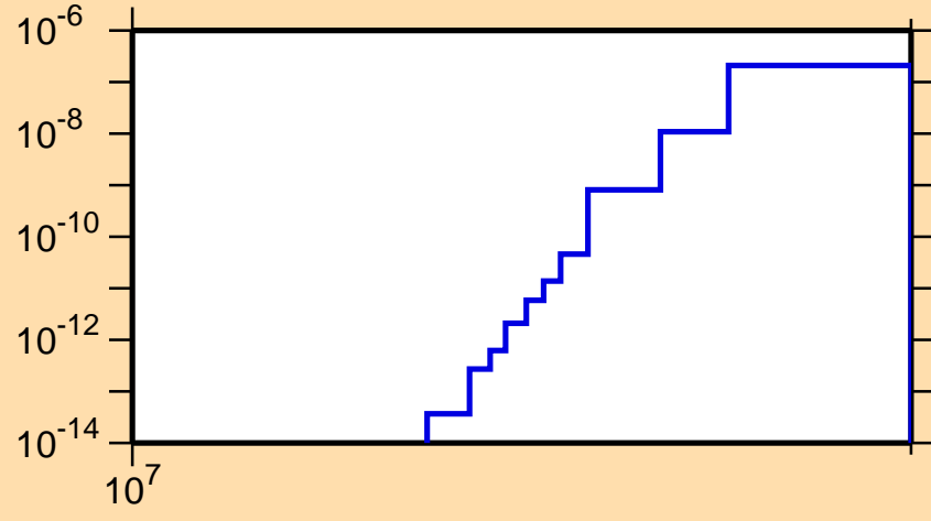
\sigma vs. E for ^{85}\text{Mo} (mt 34)
