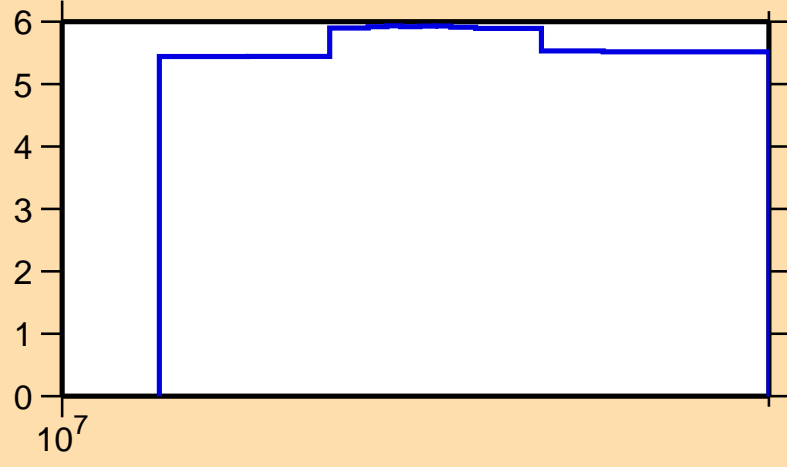
\Delta\sigma/\sigma vs. E for ^{85}\text{Mo}(n,\text{nonel.})
