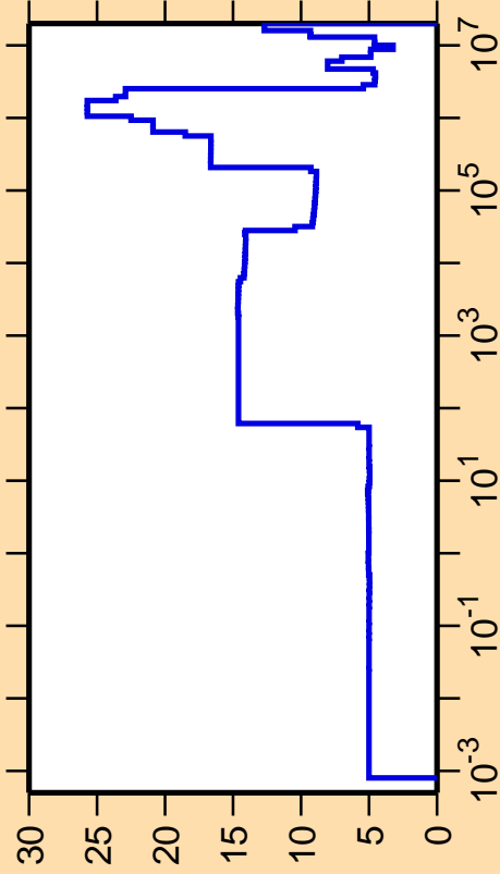
\Delta\sigma/\sigma vs. E for ^{85}\text{Mo}(n,\text{el.})
