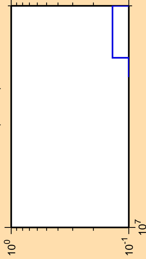
\Delta\sigma/\sigma vs. E for ^{85}\text{Mo}(n,2n\alpha)
