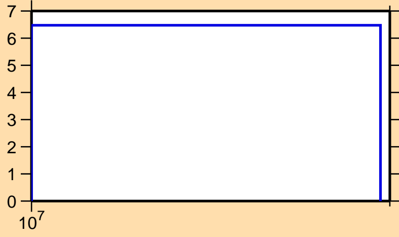
\Delta\sigma/\sigma vs. E for ^{85}\text{Mo}(n,\text{tot.})
