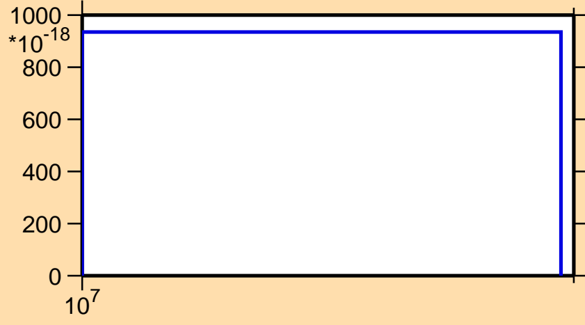
\sigma vs. E for ^{85}\text{Mo}(n,2n\alpha)
