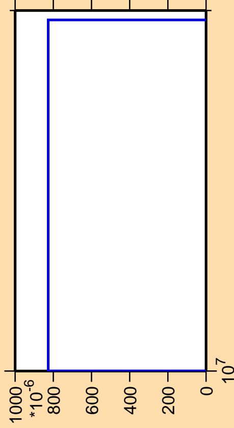
\Delta\sigma/\sigma vs. E for ^{85}\text{Mo}(n,2n\alpha)
