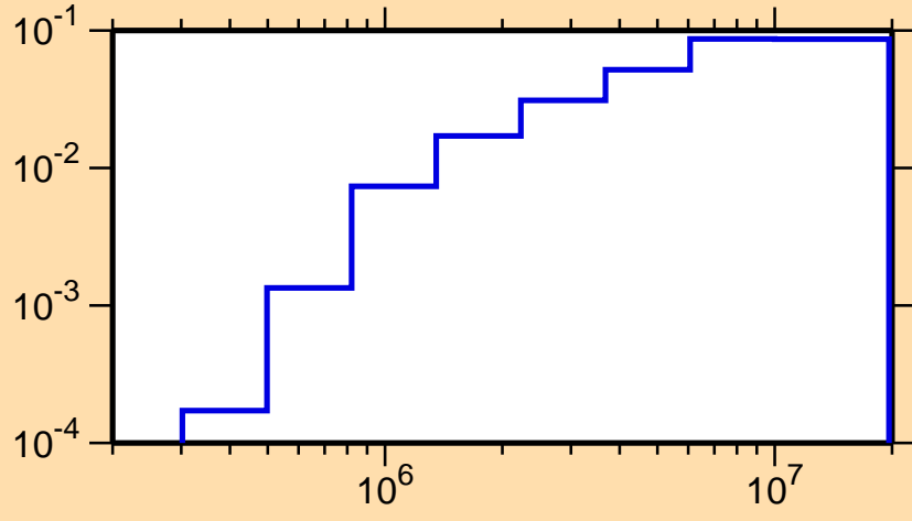
\sigma vs. E for ^{85}\text{Mo}(n,n\text{cont.})
