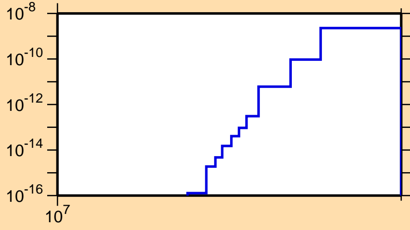
\sigma vs. E for ^{86}\text{Mo}(\text{mt117})
