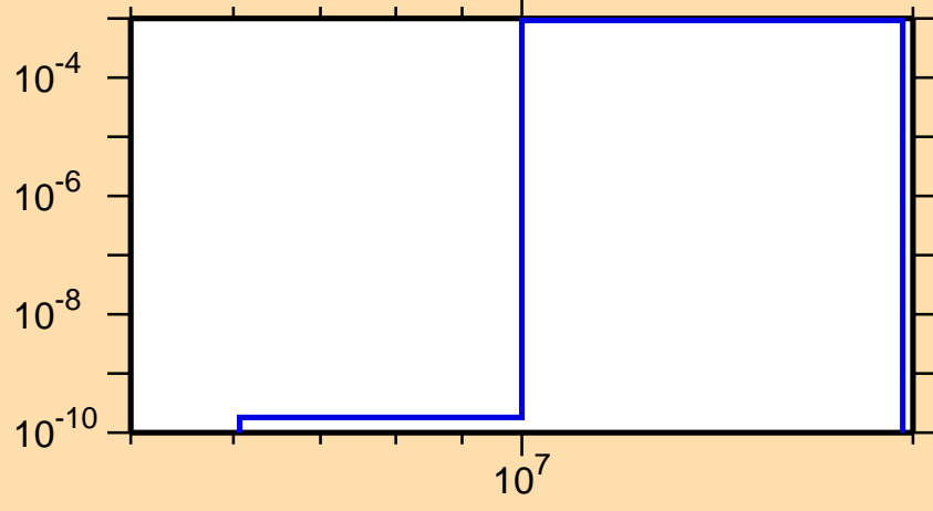
\sigma vs. E for ^{86}\text{Mo}(n,\text{pd})
