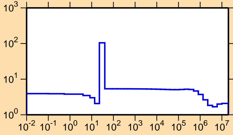
\sigma vs. E for ^{86}\text{Mo}(n,\text{el.})
