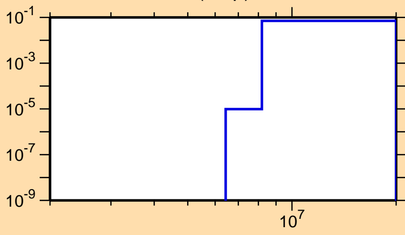
\sigma vs. E for ^{86}\text{Mo}(n,np)
