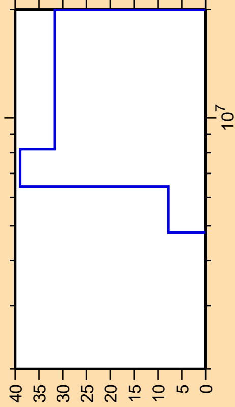
\Delta\sigma/\sigma vs. E for ^{86}\text{Mo}(n,np)
