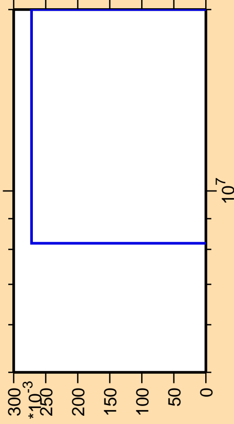
\Delta\sigma/\sigma vs. E for ^{86}\text{Mo} (mt 34)
