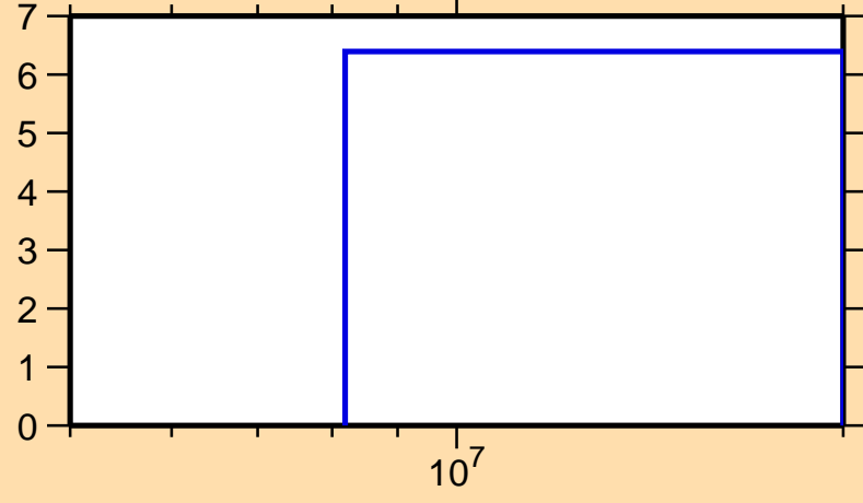
\Delta\sigma/\sigma vs. E for ^{86}\text{Mo}(n,\text{el.})
