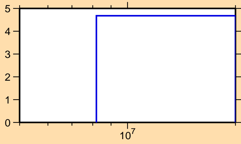
\Delta\sigma/\sigma vs. E for ^{86}\text{Mo}(n,\text{tot.})
