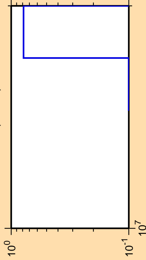
\Delta\sigma/\sigma vs. E for ^{88}\text{Mo} (mt 34)
