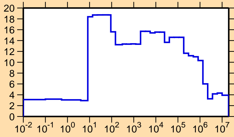
\Delta\sigma/\sigma vs. E for ^{88}\text{Mo}(n,\text{nonel.})
