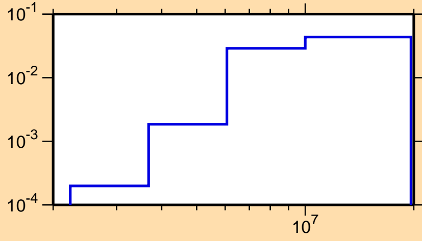
\sigma vs. E for ^{88}\text{Mo}(n,n\text{cont.})
