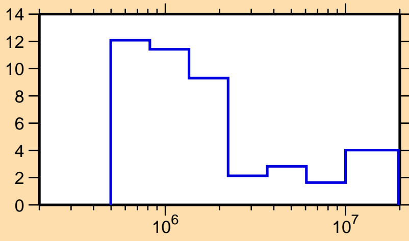
\Delta\sigma/\sigma vs. E for ^{88}\text{Mo}(n,\text{tot.})
