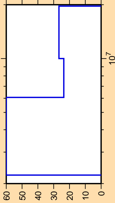
\Delta\sigma/\sigma vs. E for ^{88}\text{Mo}(n,n\text{cont.})
