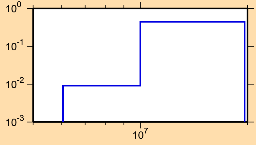
\sigma vs. E for ^{88}\text{Mo}(n,np)
