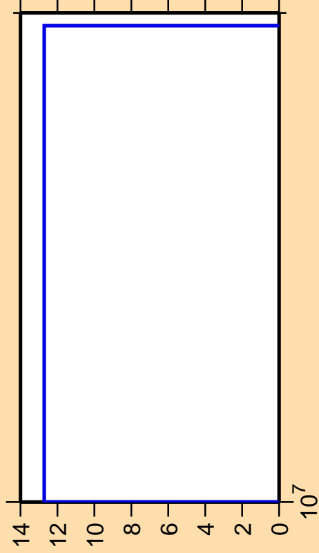
\Delta\sigma/\sigma vs. E for ^{88}\text{Mo} (mt 45)
