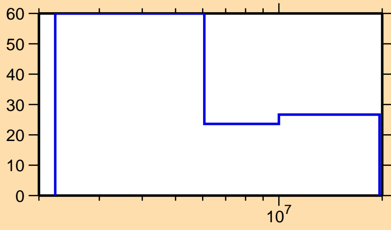
\Delta\sigma/\sigma vs. E for ^{88}\text{Mo}(n,n\text{cont.})
