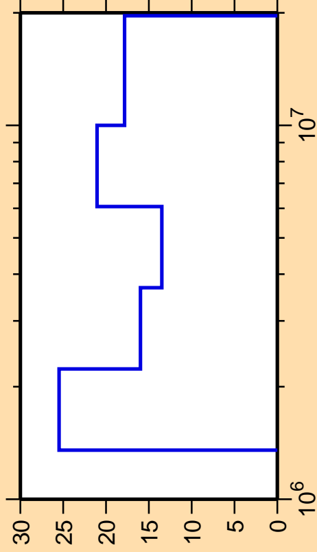
\Delta\sigma/\sigma vs. E for ^{88}\text{Mo}(n,n_3)
