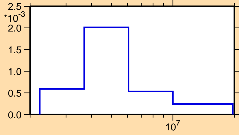
\sigma vs. E for ^{88}\text{Mo}(n,n_4)
