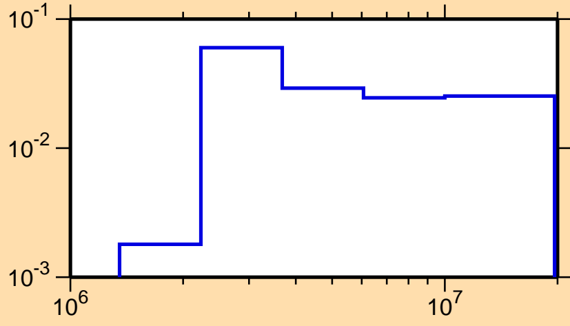
\sigma vs. E for ^{88}\text{Mo}(n,n_3)
