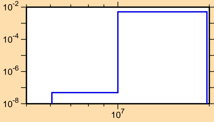
\sigma vs. E for ^{88}\text{Mo}(n,p\alpha)
