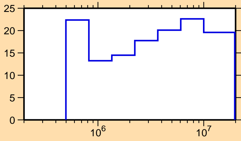
\Delta\sigma/\sigma vs. E for ^{88}\text{Mo}(n,n_1)
