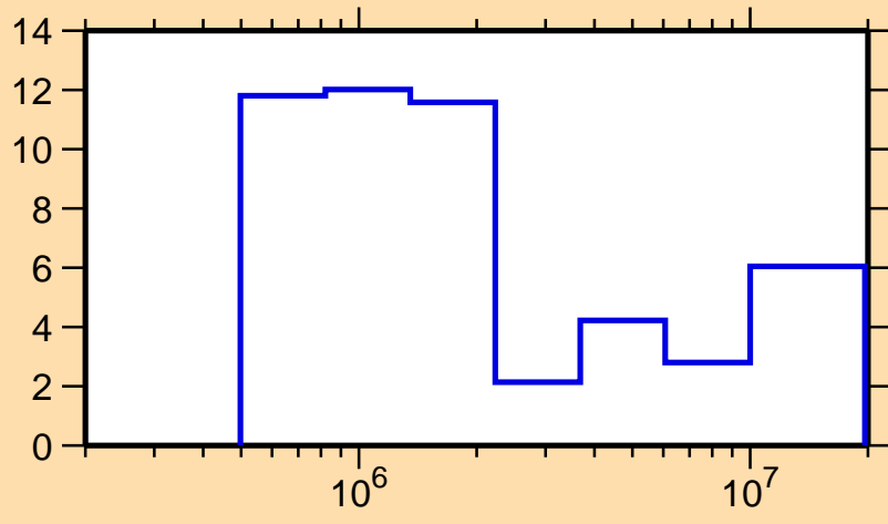
\Delta\sigma/\sigma vs. E for ^{88}\text{Mo}(n,\text{el.})
