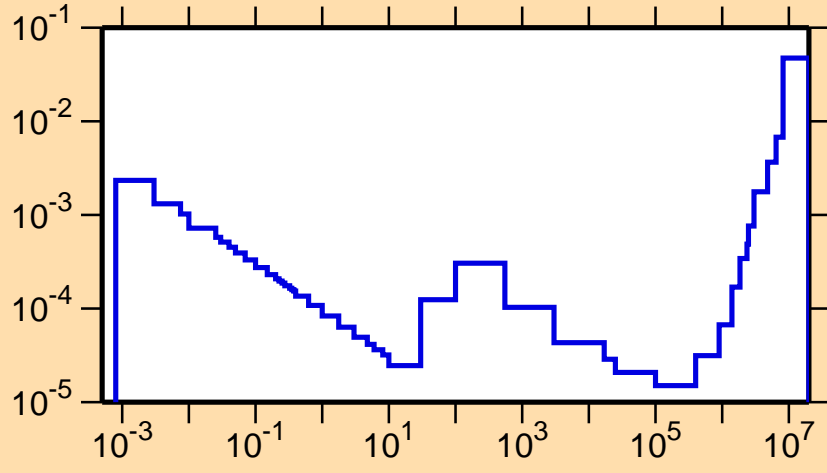
\sigma vs. E for ^{88}\text{Mo}(n,\alpha)
