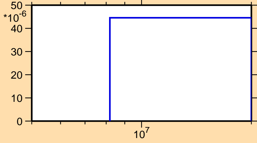
\sigma vs. E for ^{88}\text{Mo}(n,pd)
