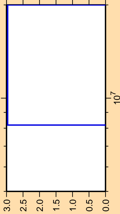
\Delta\sigma/\sigma vs. E for ^{88}\text{Mo}(\text{mt117})
