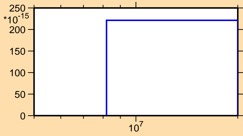
\sigma vs. E for ^{88}\text{Mo}(n,nd)
