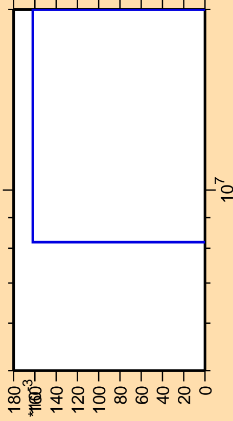
\Delta\sigma/\sigma vs. E for ^{88}\text{Mo}(n,nd)
