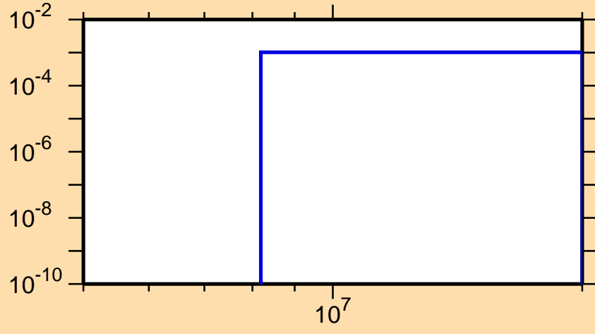
\sigma vs. E for ^{88}\text{Mo}(n,n\alpha)
