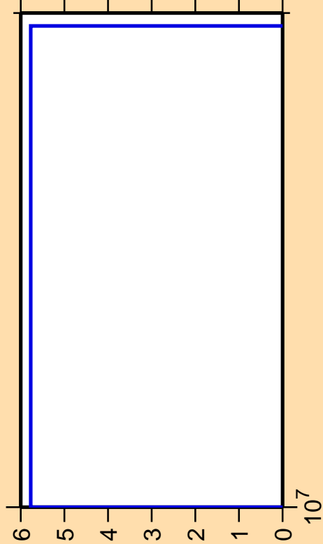
\Delta\sigma/\sigma vs. E for ^{89}\text{Mo}(n,n_1)
