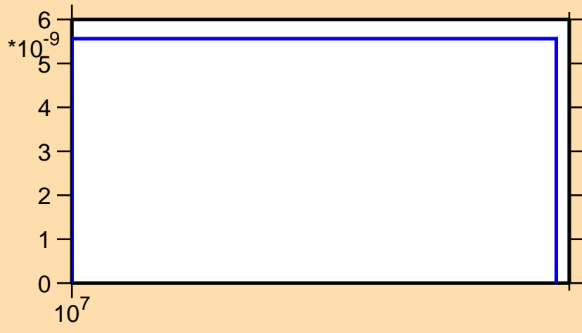
\sigma vs. E for ^{89}\text{Mo}(n,\text{pt})
