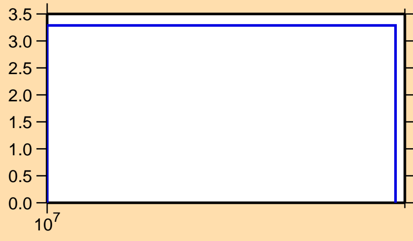
\Delta\sigma/\sigma vs. E for ^{89}\text{Mo}(n,\text{tot.})
