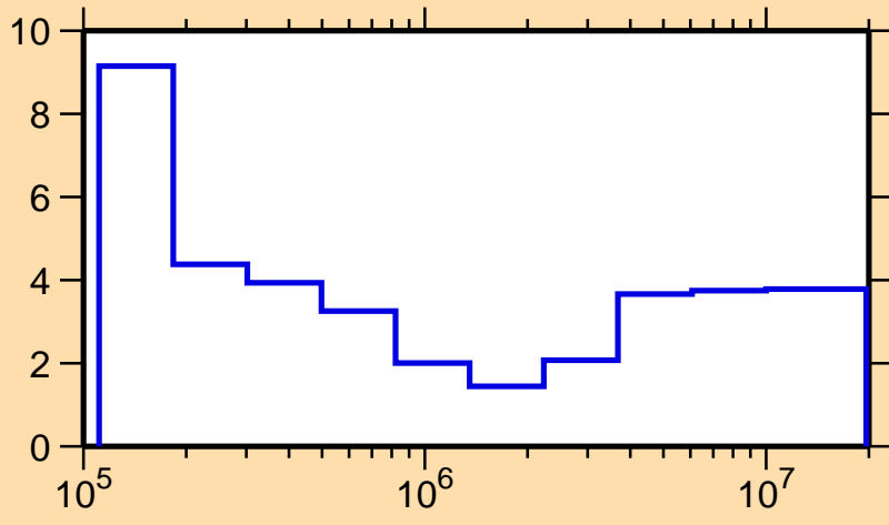
\Delta\sigma/\sigma vs. E for ^{89}\text{Mo}(n,\text{nonel.})
