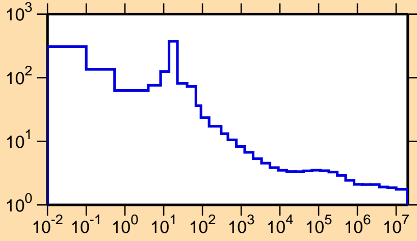
\sigma vs. E for ^{89}\text{Mo}(n,\text{nonel.})
