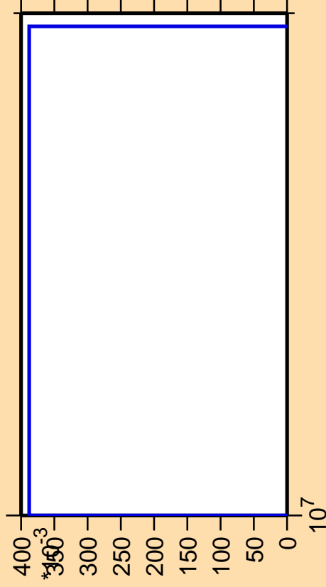
\Delta\sigma/\sigma vs. E for ^{89}\text{Mo} (mt 45)
