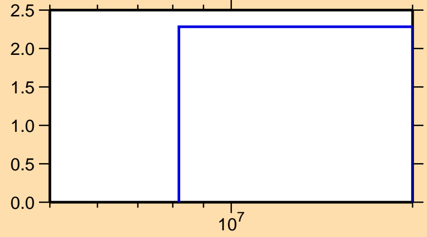
\Delta\sigma/\sigma vs. E for ^{89}\text{Mo}(n,\text{el.})
