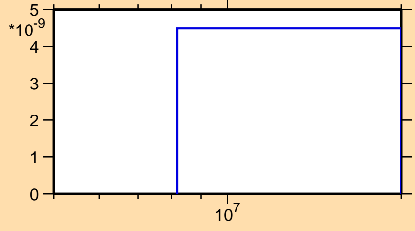
\sigma vs. E for ^{89}\text{Mo}(n,nd)
