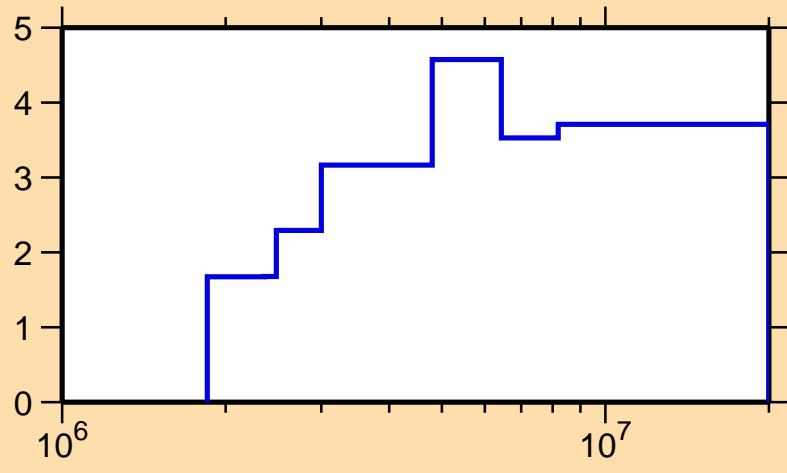
\Delta\sigma/\sigma vs. E for ^{89}\text{Mo}(n,\text{nonel.})
