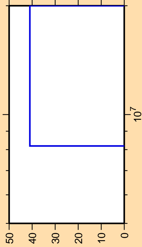
\Delta\sigma/\sigma vs. E for ^{89}\text{Mo}(n,nd)
