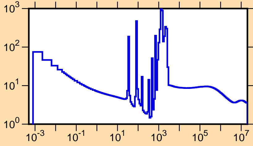
\sigma vs. E for ^{90}\text{Mo}(n,\text{tot.})
