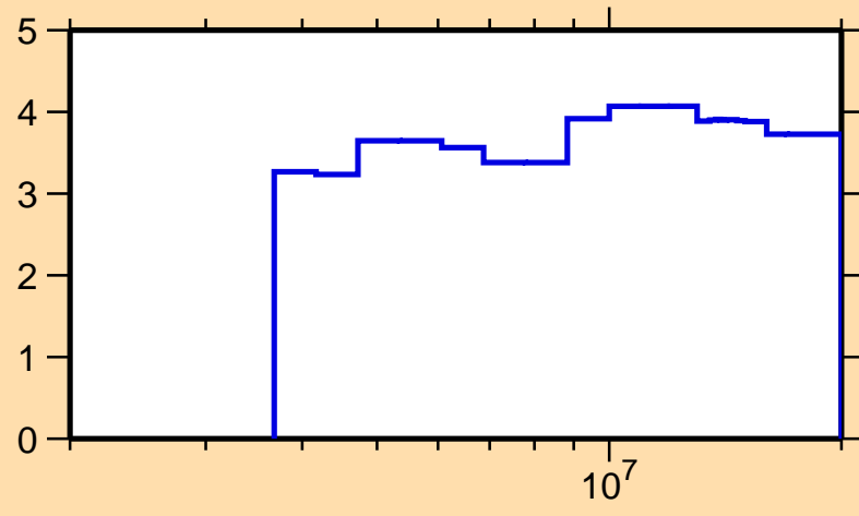
\Delta\sigma/\sigma vs. E for ^{90}\text{Mo}(n,n\text{onel.})
