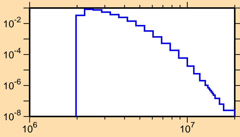
\sigma vs. E for ^{90}\text{Mo}(n,n_3)
