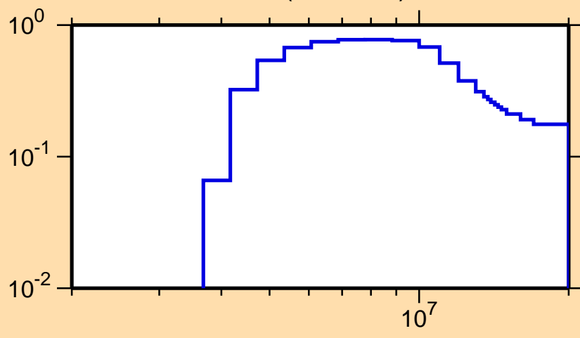
\sigma vs. E for ^{90}\text{Mo}(n,n\text{cont.})
