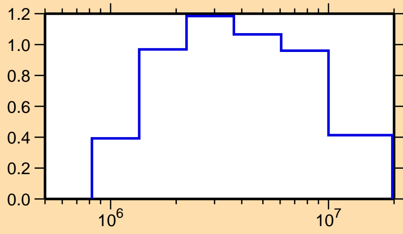
\sigma vs. E for ^{90}\text{Mo}(n,\text{inel.})
