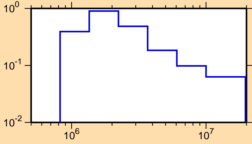
\sigma vs. E for ^{90}\text{Mo}(n,n_1)
