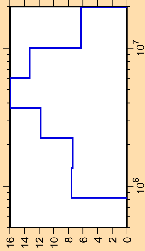
\Delta\sigma/\sigma vs. E for ^{90}\text{Mo}(n,\text{inel.})
