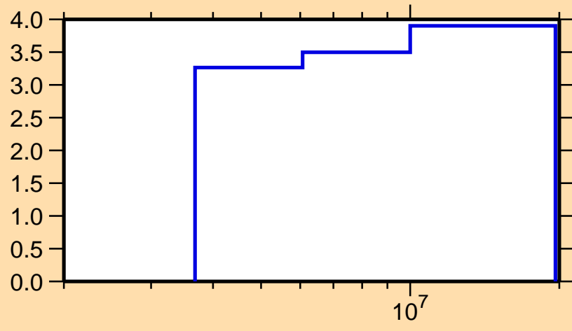
\Delta\sigma/\sigma vs. E for ^{90}\text{Mo}(n,n\text{onel.})
