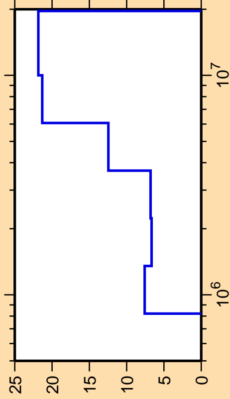
\Delta\sigma/\sigma vs. E for ^{90}\text{Mo}(n,n_1)
