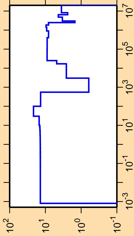
\Delta\sigma/\sigma vs. E for ^{90}\text{Mo}(n,\text{el.})
