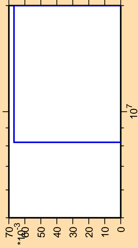
\Delta\sigma/\sigma vs. E for ^{90}\text{Mo}(n,nd)
