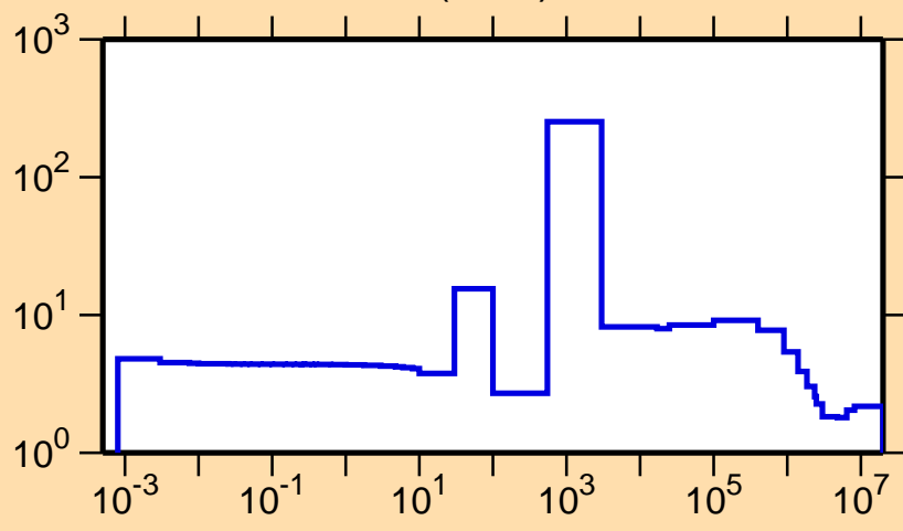
\sigma vs. E for ^{90}\text{Mo}(n,\text{el.})
