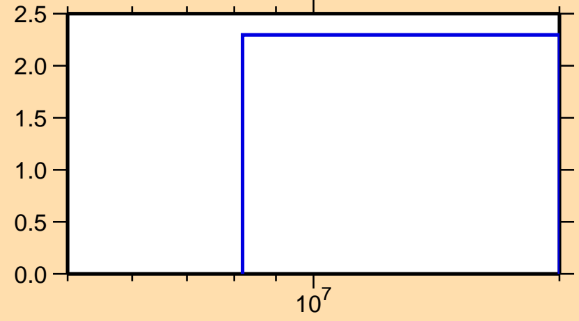
\Delta\sigma/\sigma vs. E for ^{90}\text{Mo}(n,\text{tot.})
