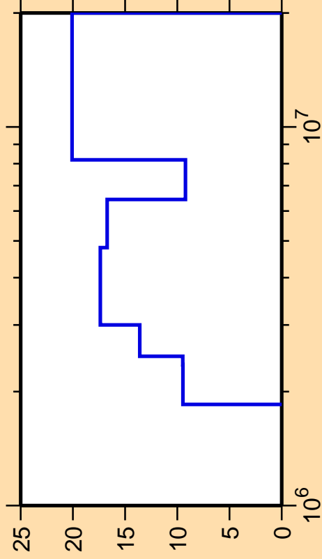
\Delta\sigma/\sigma vs. E for ^{90}\text{Mo}(n,n_2)
