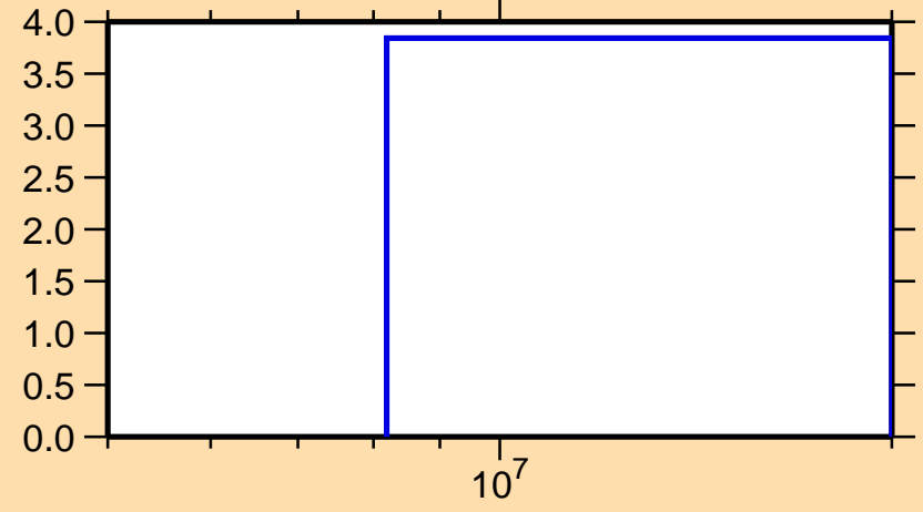
\Delta\sigma/\sigma vs. E for ^{90}\text{Mo}(n,\text{nonel.})
