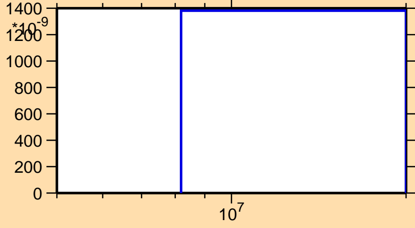
\sigma vs. E for ^{90}\text{Mo}(n,t)
