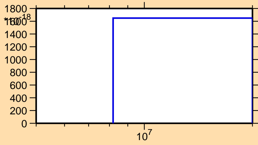
\sigma vs. E for ^{90}\text{Mo}(\text{mt117})
