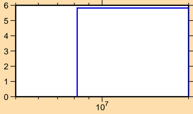
\Delta\sigma/\sigma vs. E for ^{90}\text{Mo}(n,\text{inel.})
