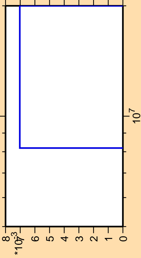
\Delta\sigma/\sigma vs. E for ^{90}\text{Mo} (mt 45)
