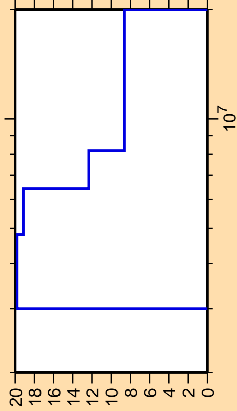
\Delta\sigma/\sigma vs. E for ^{90}\text{Mo}(n,p)
