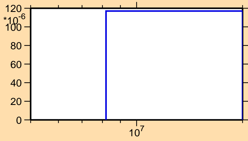
\sigma vs. E for ^{90}\text{Mo}(n,p\alpha)
