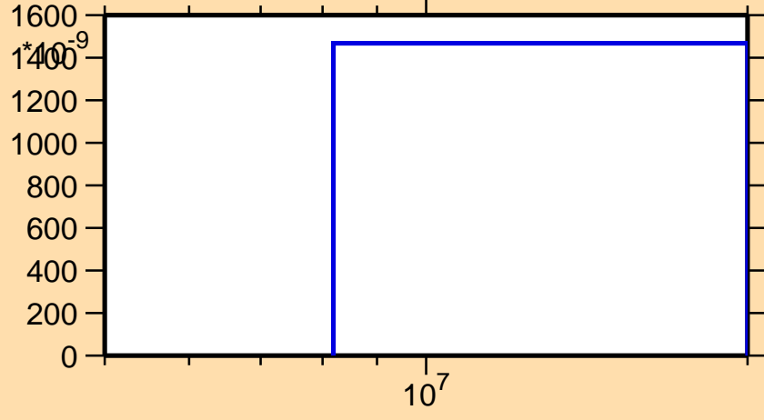
\sigma vs. E for ^{90}\text{Mo}(n,pd)
