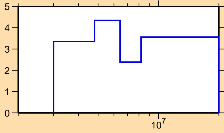
\Delta\sigma/\sigma vs. E for ^{90}\text{Mo}(n,\text{el.})
