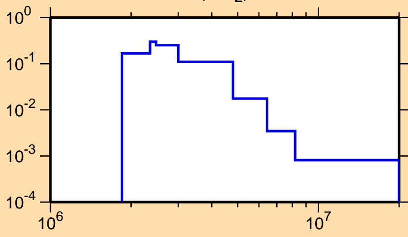
\sigma vs. E for ^{90}\text{Mo}(n,n_2)
