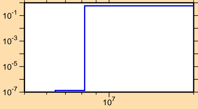
\sigma vs. E for ^{90}\text{Mo}(n,np)
