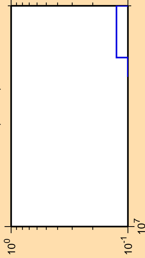
\Delta\sigma/\sigma vs. E for ^{91}\text{Mo} (mt 45)
