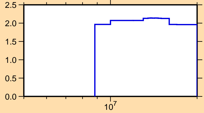
\Delta\sigma/\sigma vs. E for ^{91}\text{Mo}(n,\text{nonel.})
