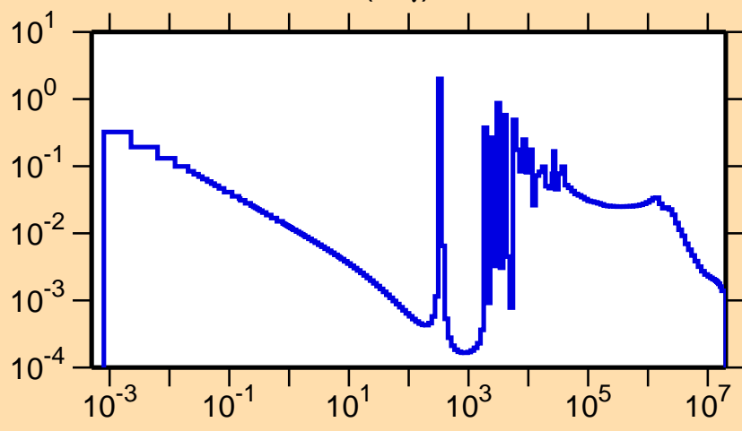
\sigma vs. E for ^{92}\text{Mo}(n,\gamma)
