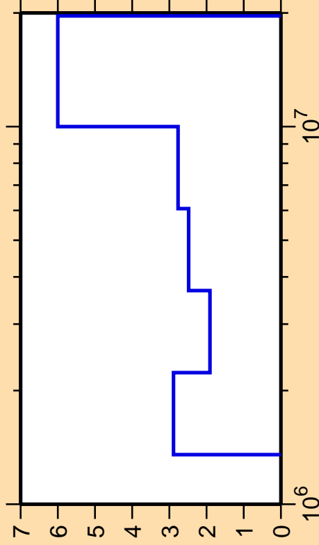
\Delta\sigma/\sigma vs. E for ^{92}\text{Mo}(n,\text{inel.})
