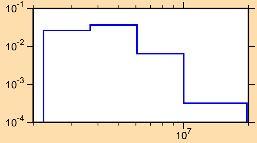
\sigma vs. E for ^{92}\text{Mo}(n,n_4)
