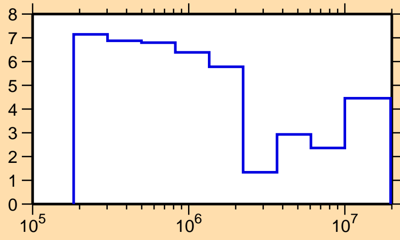
\Delta\sigma/\sigma vs. E for ^{92}\text{Mo}(n,el.)
