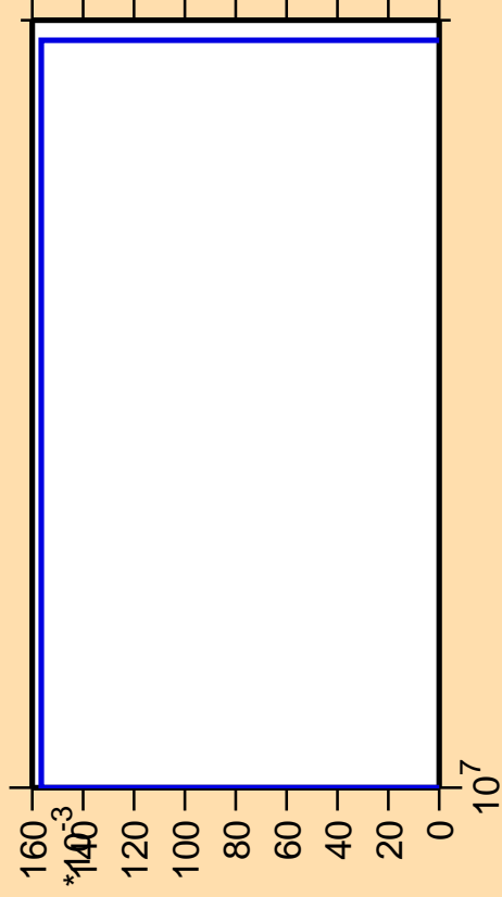
\Delta\sigma/\sigma vs. E for ^{92}\text{Mo}(n,\text{nd})
