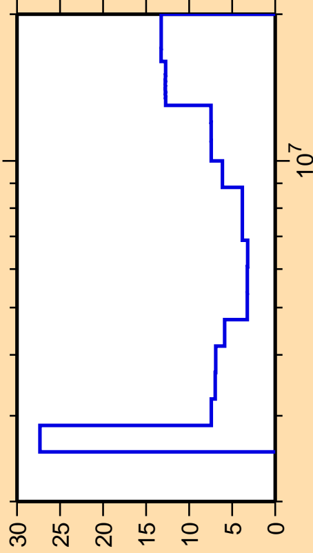
\Delta\sigma/\sigma vs. E for ^{93}\text{Mo}(n,n_{\text{cont}})
