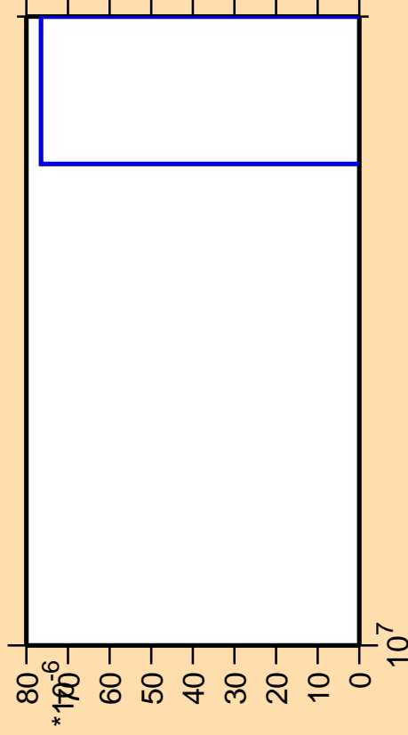
\Delta\sigma/\sigma vs. E for ^{93}\text{Mo}(n,nt)
