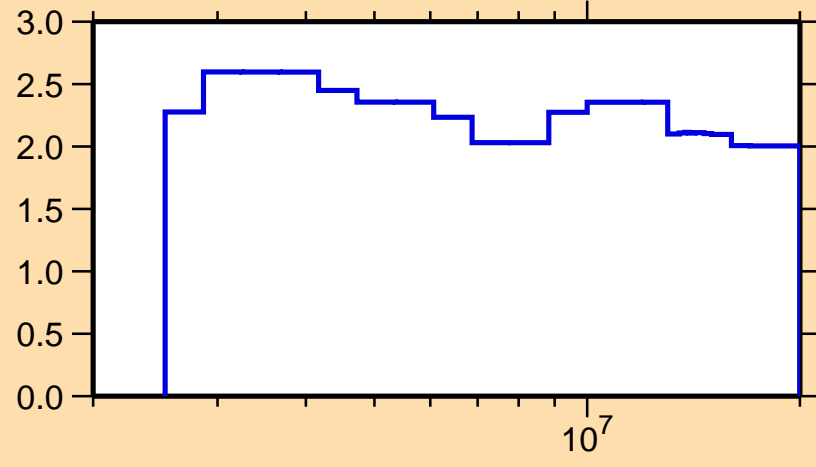
\Delta\sigma/\sigma vs. E for ^{93}\text{Mo}(n,n\text{onel.})
