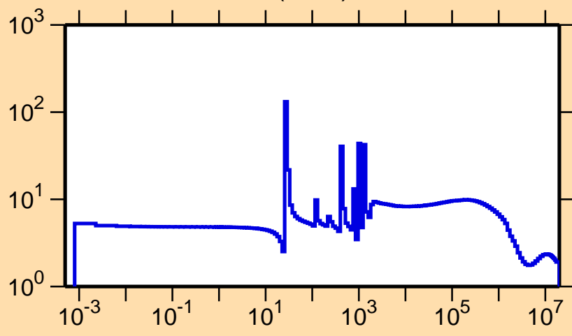
\sigma vs. E for ^{93}\text{Mo}(n,\text{el.})
