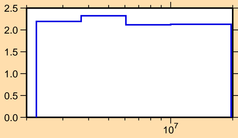
\Delta\sigma/\sigma vs. E for ^{93}\text{Mo}(n,n\text{nonel.})
