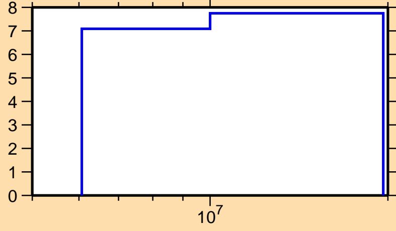
\Delta\sigma/\sigma vs. E for ^{93}\text{Mo}(n,2n)
