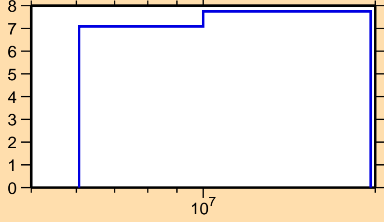
\Delta\sigma/\sigma vs. E for ^{93}\text{Mo}(n,2n)
