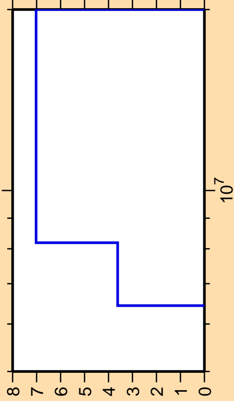
\Delta\sigma/\sigma vs. E for ^{93}\text{Mo}(n,n\text{cont.})
