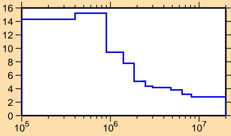
\Delta\sigma/\sigma vs. E for ^{93}\text{Mo}(n,n\text{onel.})
