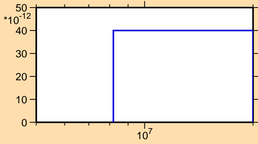
\sigma vs. E for ^{93}\text{Mo}(\text{mt } 34)
