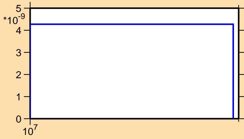
\sigma vs. E for ^{94}\text{Mo}(n,\text{nd})
