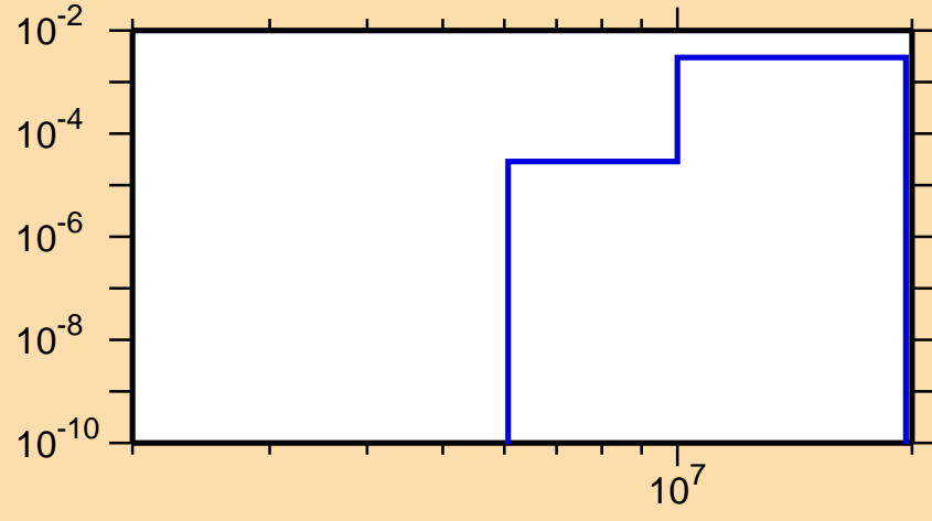
\sigma vs. E for ^{94}\text{Mo}(n,n\alpha)
