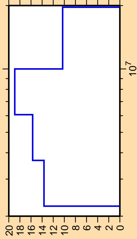
\Delta\sigma/\sigma vs. E for ^{94}\text{Mo}(n,p)
