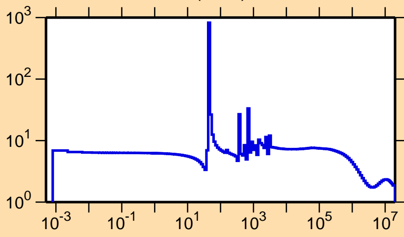
\sigma vs. E for ^{95}\text{Mo}(n,\text{el.})
