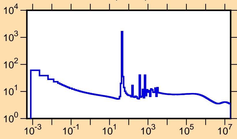
\sigma vs. E for ^{95}\text{Mo}(n,\text{tot.})
