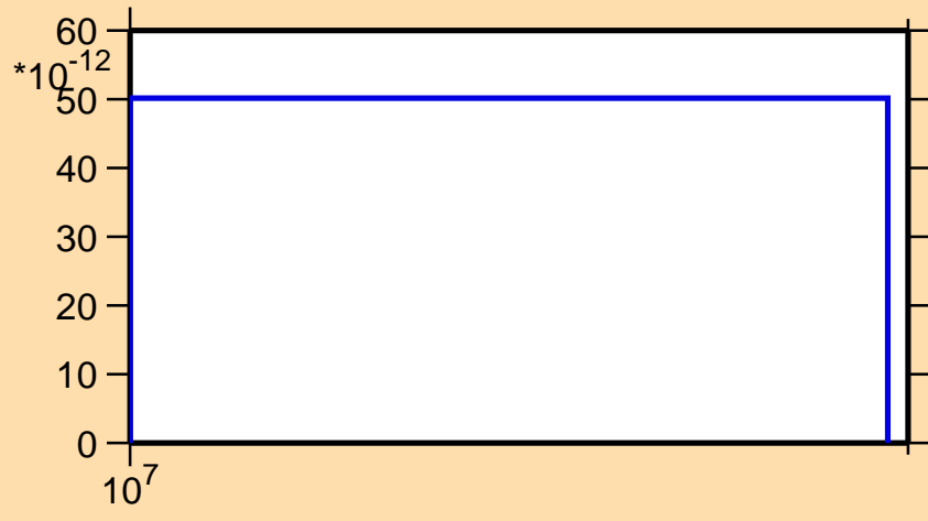
\sigma vs. E for ^{96}\text{Mo}(n,p\alpha)
