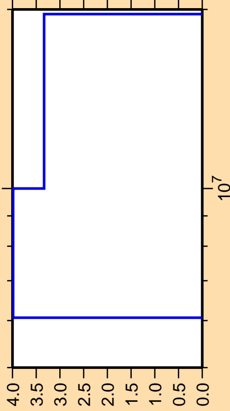
\Delta\sigma/\sigma vs. E for ^{96}\text{Mo}(n,2n)
