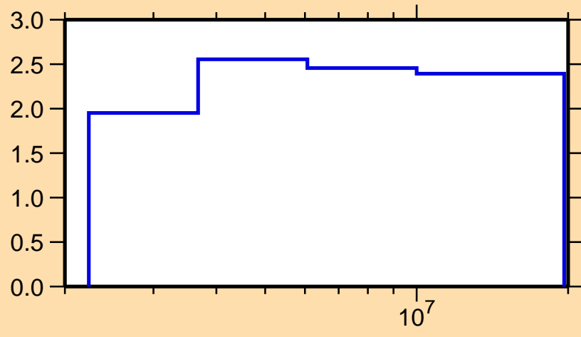
\Delta\sigma/\sigma vs. E for ^{96}\text{Mo}(n,n\text{onel.})
