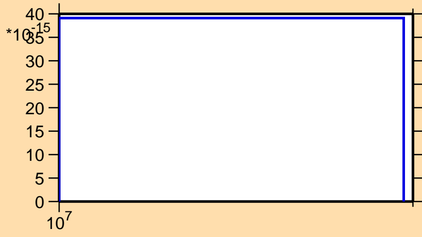
\sigma vs. E for ^{96}\text{Mo}(n,\text{pd})
