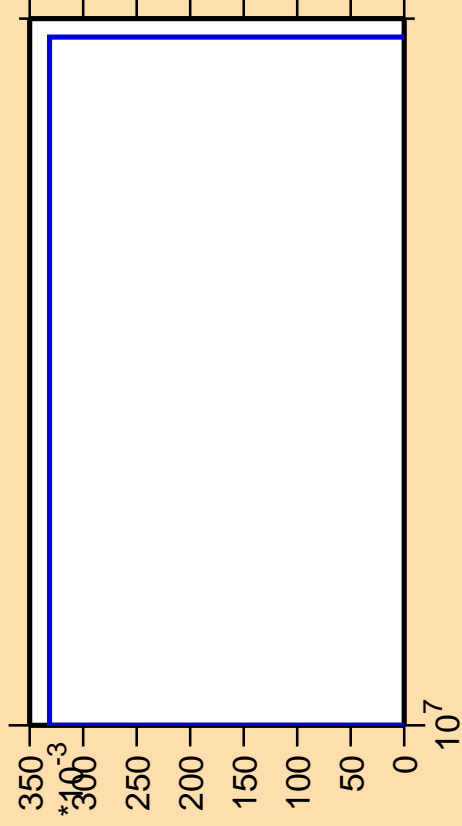
\Delta\sigma/\sigma vs. E for ^{96}\text{Mo}(n,2np)
