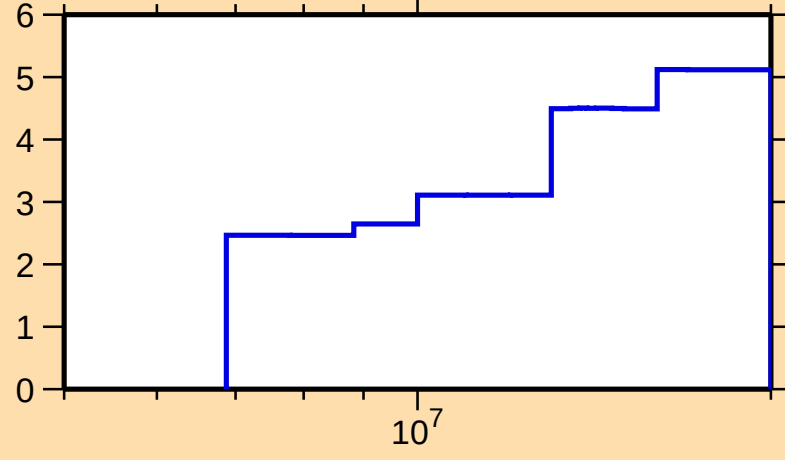
\Delta\sigma/\sigma vs. E for ^{97}\text{Mo}(n,\text{el.})
