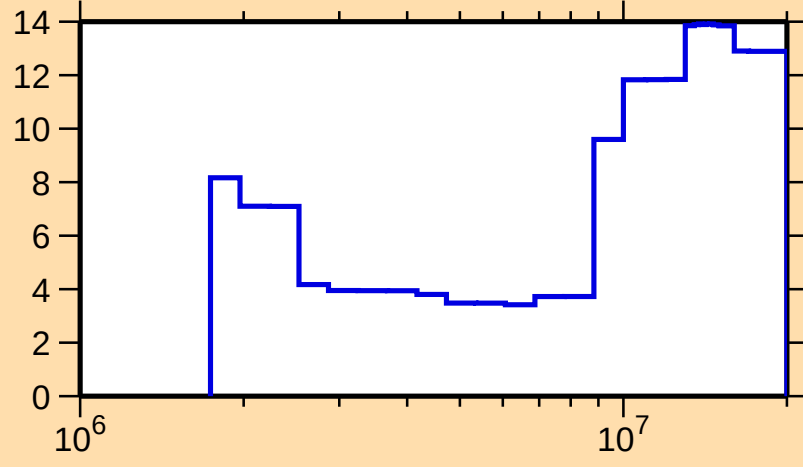
\Delta\sigma/\sigma vs. E for ^{97}\text{Mo}(n,n\text{cont.})
