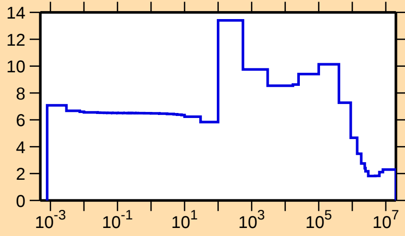
\sigma vs. E for ^{97}\text{Mo}(n,\text{el.})
