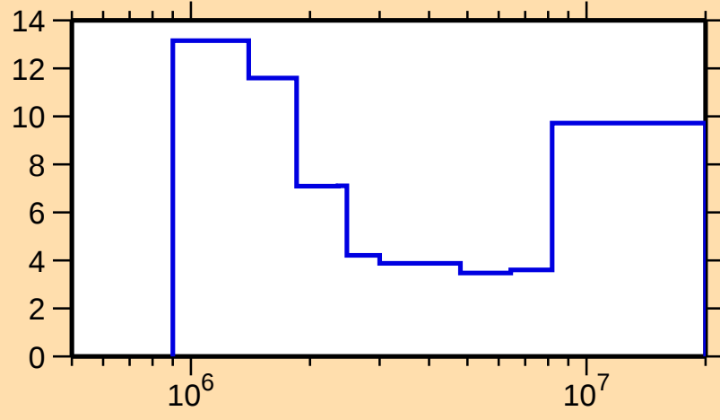
\Delta\sigma/\sigma vs. E for ^{97}\text{Mo}(n,n\text{cont.})
