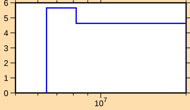
\Delta\sigma/\sigma vs. E for ^{97}\text{Mo}(n,2n)
