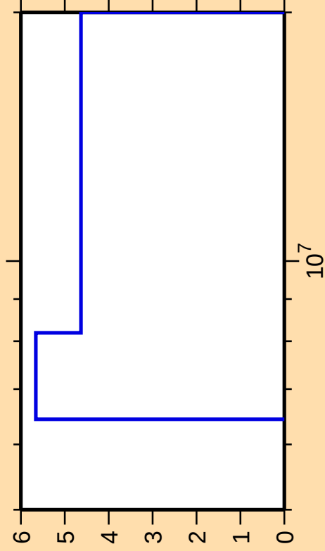
\Delta\sigma/\sigma vs. E for ^{97}\text{Mo}(n,2n)
