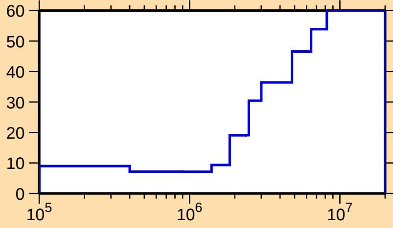
\Delta\sigma/\sigma vs. E for ^{97}\text{Mo}(n,n_1)
