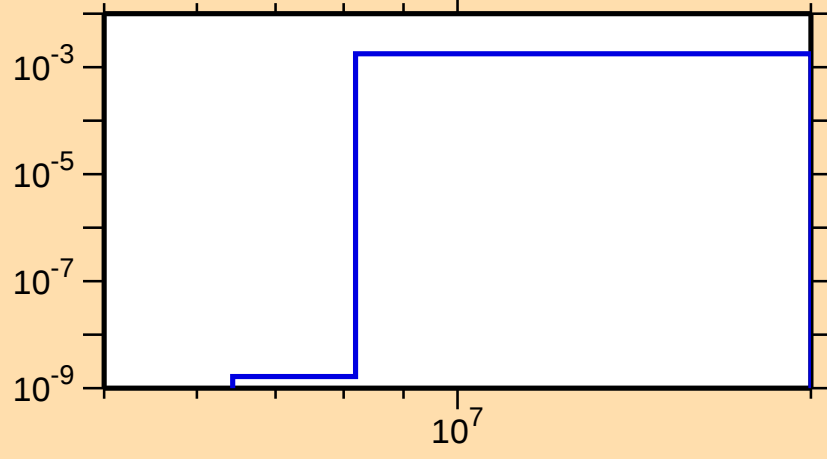
\sigma vs. E for ^{97}\text{Mo}(n,n\alpha)
