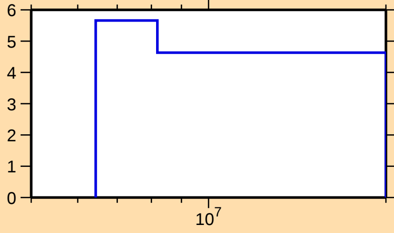
\Delta\sigma/\sigma vs. E for ^{97}\text{Mo}(n,2n)
