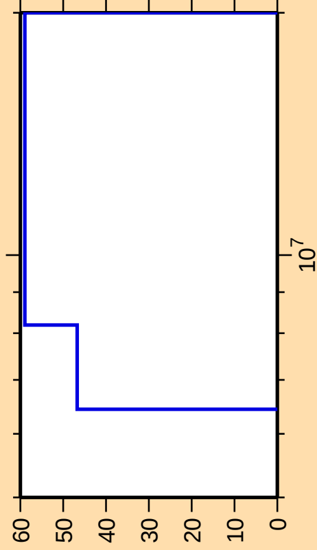
\Delta\sigma/\sigma vs. E for ^{97}\text{Mo}(n,n\alpha)
