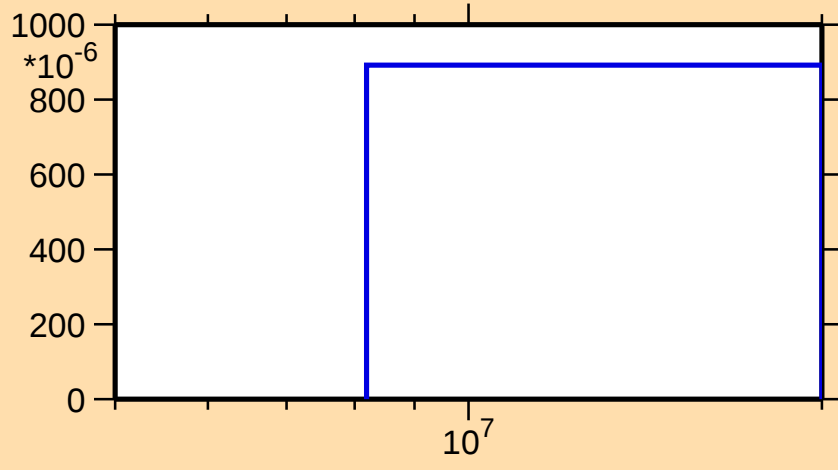
\sigma vs. E for ^{97}\text{Mo}(n,d)
