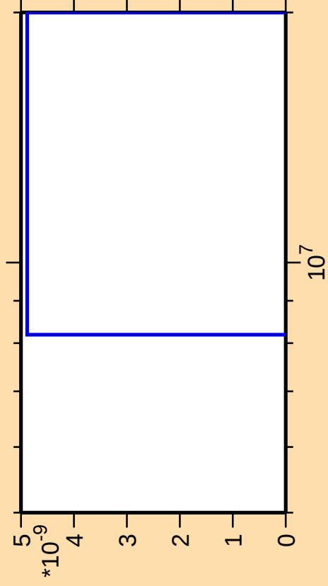
\Delta\sigma/\sigma vs. E for ^{97}\text{Mo}(n,3n\alpha)
