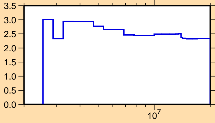
\Delta\sigma/\sigma vs. E for ^{98}\text{Mo}(n,n\text{onel.})
