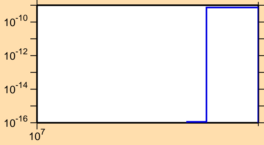
\sigma vs. E for ^{98}\text{Mo}(n,nt)
