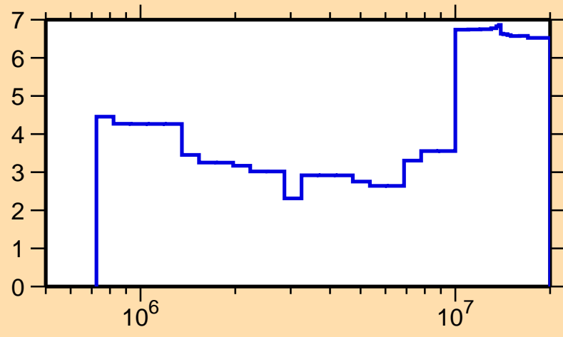
\Delta\sigma/\sigma vs. E for ^{98}\text{Mo}(n,\text{inel.})
