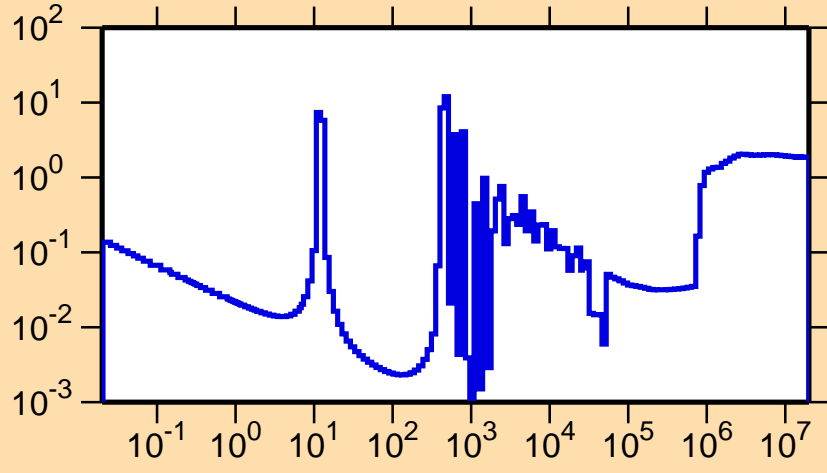
\sigma vs. E for ^{98}\text{Mo}(n,\text{nonel.})
