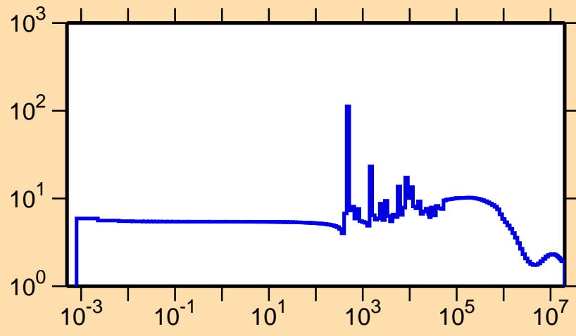
\sigma vs. E for ^{98}\text{Mo}(n,\text{el.})
