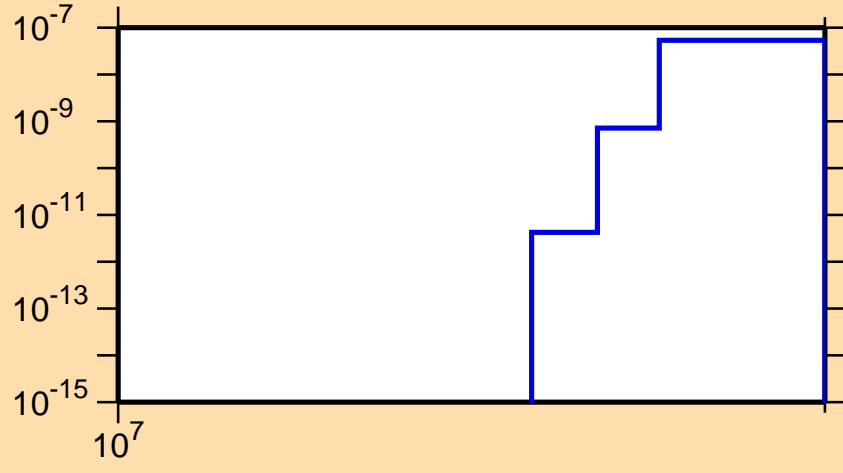
\sigma vs. E for ^{98}\text{Mo}(n,2n\alpha)
