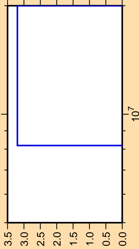
\Delta\sigma/\sigma vs. E for ^{98}\text{Mo}(n,2n)
