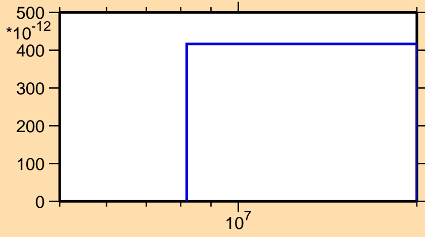
\sigma vs. E for ^{98}\text{Mo}(n,nd)
