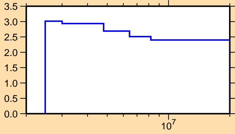
\Delta\sigma/\sigma vs. E for ^{98}\text{Mo}(n,n\text{onl.})
