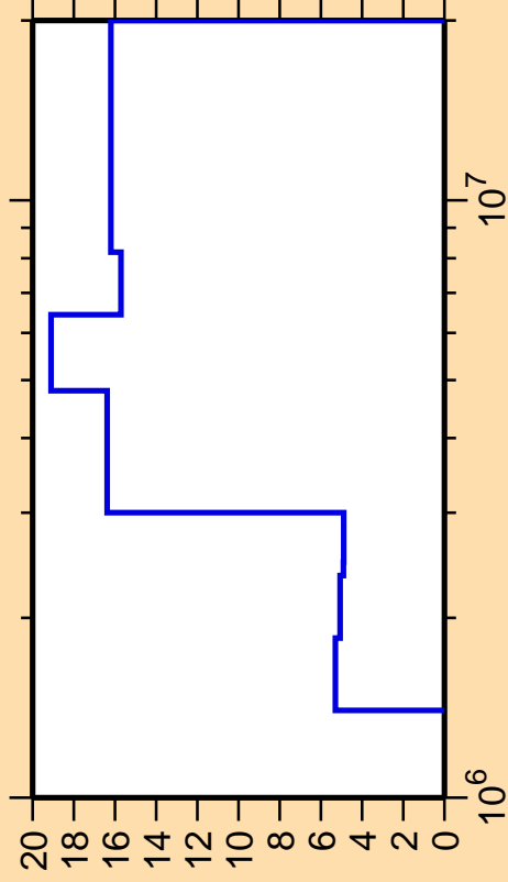
\Delta\sigma/\sigma vs. E for ^{98}\text{Mo}(n,n_3)
