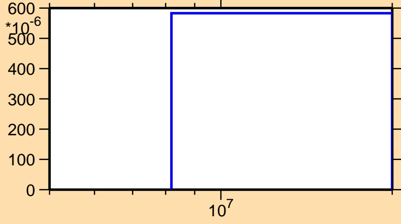
\sigma vs. E for ^{98}\text{Mo}(n,d)
