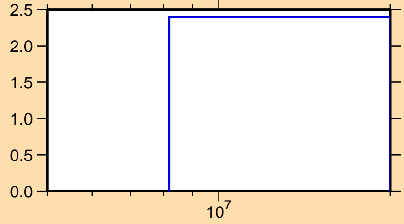
\Delta\sigma/\sigma vs. E for ^{98}\text{Mo}(n,\text{nonel.})
