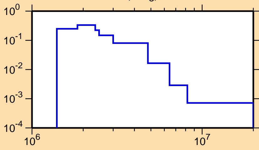
\sigma vs. E for ^{98}\text{Mo}(n,n_3)
