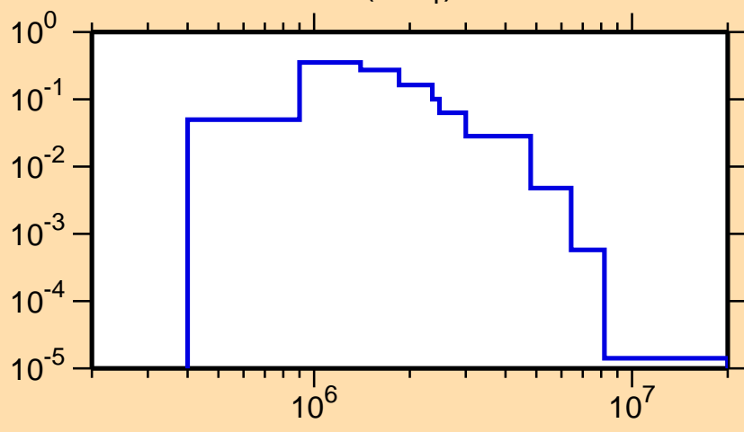
\sigma vs. E for ^{98}\text{Mo}(n,n_1)
