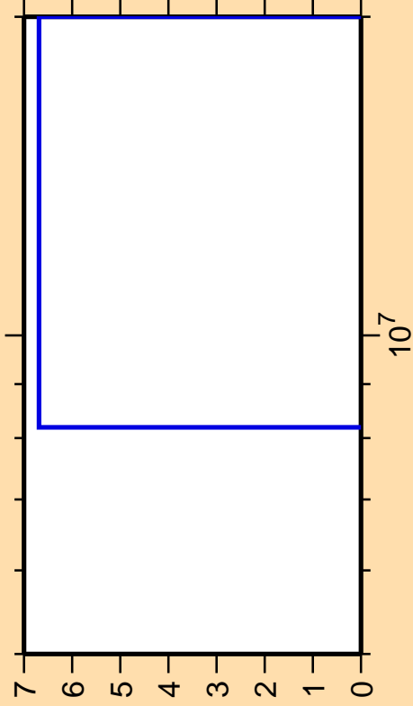
\Delta\sigma/\sigma vs. E for ^{98}\text{Mo}(n,nt)
