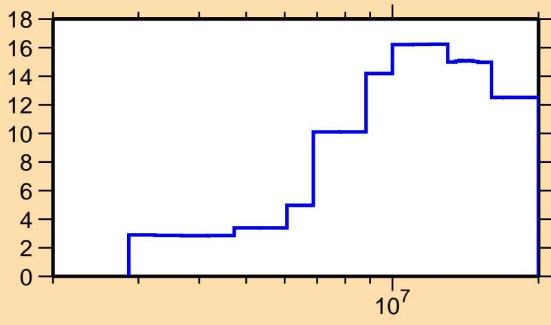
\Delta\sigma/\sigma vs. E for ^{99}\text{Mo}(n,n\text{cont.})
