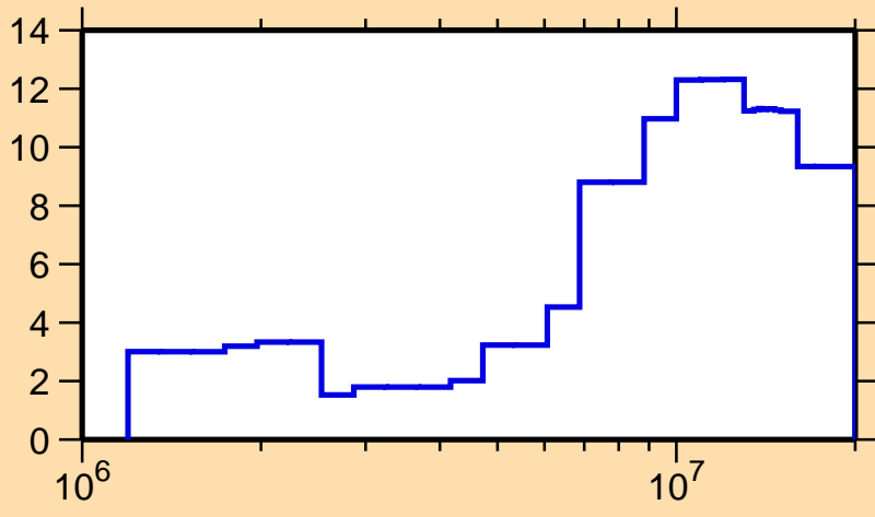
\Delta\sigma/\sigma vs. E for ^{99}\text{Mo}(n,\text{inel.})
