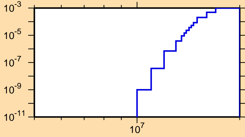
\sigma vs. E for ^{99}\text{Mo}(n,t)
