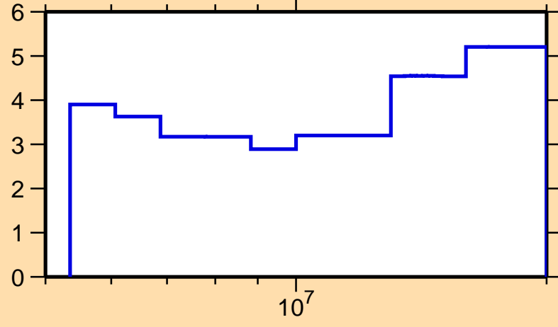
\Delta\sigma/\sigma vs. E for ^{99}\text{Mo}(n,\text{el.})
