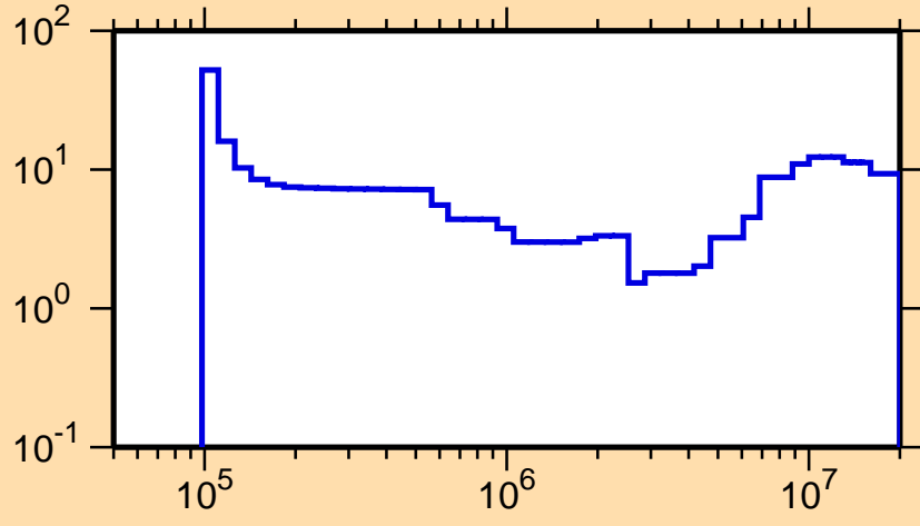
\Delta\sigma/\sigma vs. E for ^{99}\text{Mo}(n,\text{inel.})
