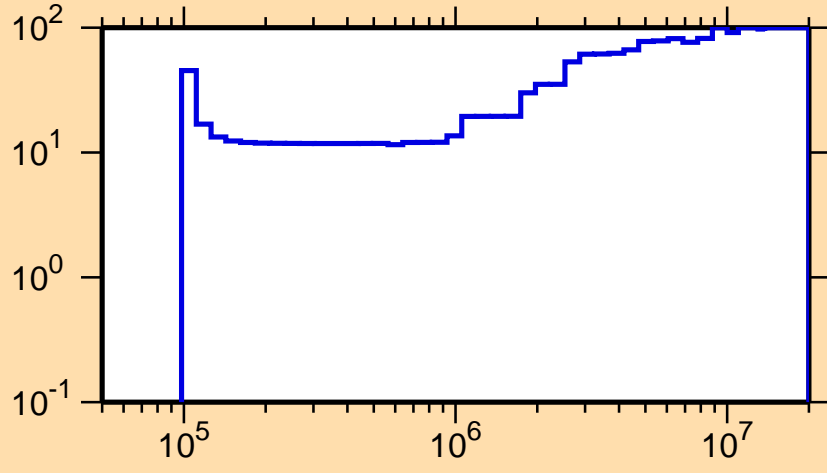
\Delta\sigma/\sigma vs. E for ^{99}\text{Mo}(n,n_1)
