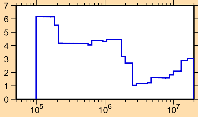
\Delta\sigma/\sigma vs. E for ^{99}\text{Mo}(n,\text{tot.})
