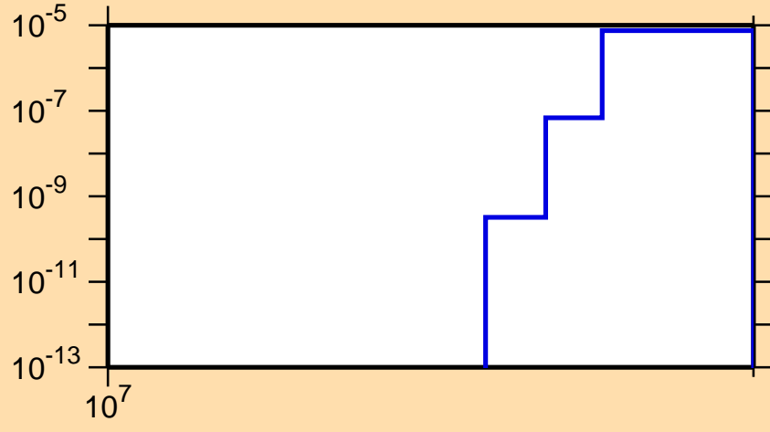
\sigma vs. E for ^{99}\text{Mo}(n,\text{nd})
