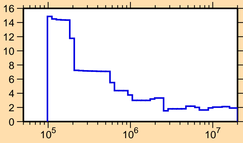
\Delta\sigma/\sigma vs. E for ^{99}\text{Mo}(n,\text{nonel.})
