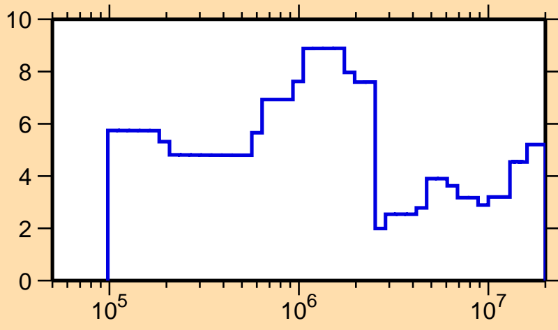
\Delta\sigma/\sigma vs. E for ^{99}\text{Mo}(n,\text{el.})
