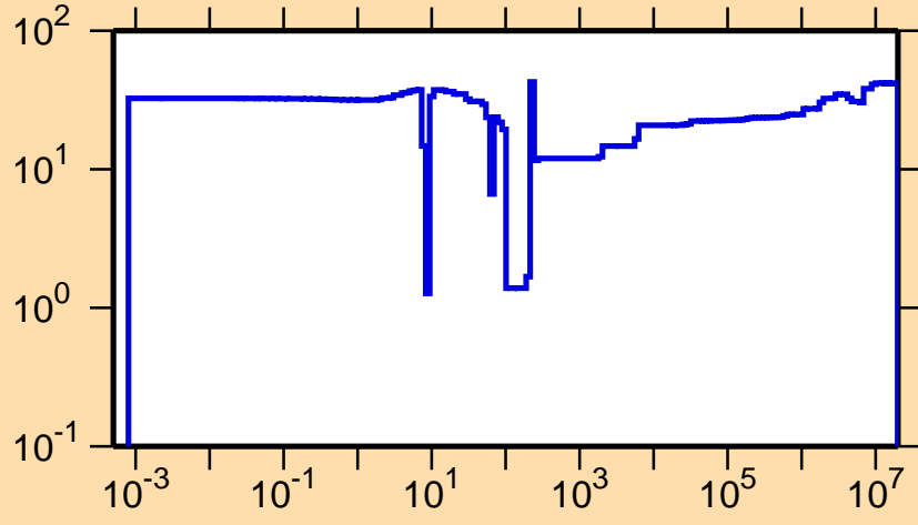
\Delta\sigma/\sigma vs. E for ^{99}\text{Mo}(n,\gamma)
