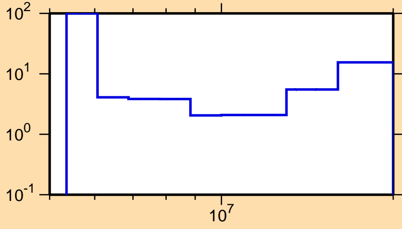
\Delta\sigma/\sigma vs. E for ^{99}\text{Mo}(n,2n)
