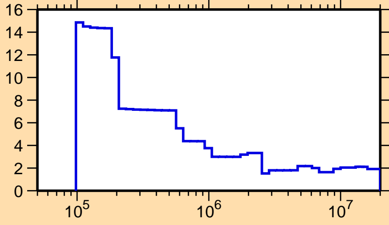
\Delta\sigma/\sigma vs. E for ^{99}\text{Mo}(n,\text{nonel.})
