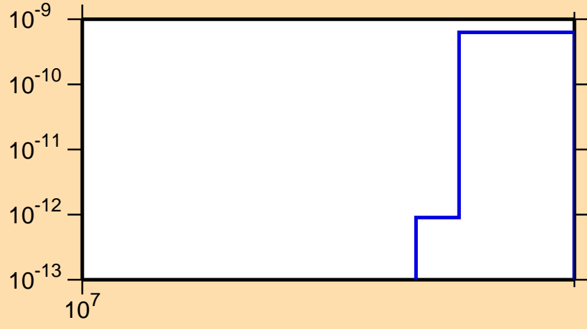
\sigma vs. E for ^{99}\text{Mo}(n,\text{He3})
