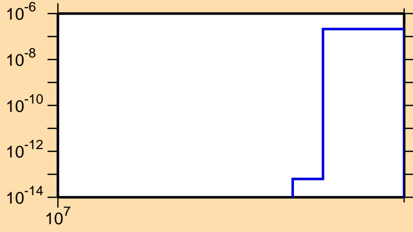
\sigma vs. E for ^{99}\text{Mo}(n,2np)
