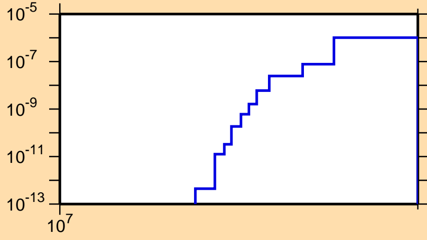
\sigma vs. E for ^{99}\text{Mo}(n,2n\alpha)
