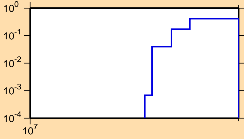
\sigma vs. E for ^{99}\text{Mo}(n,3n)
