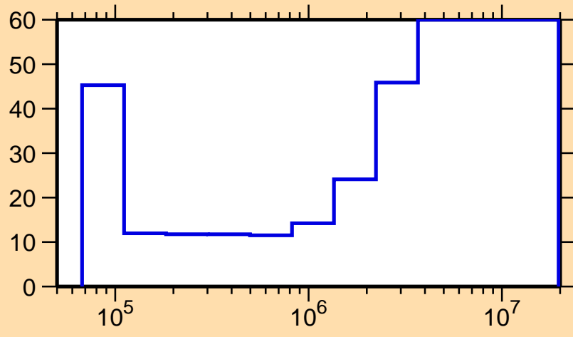
\Delta\sigma/\sigma vs. E for ^{99}\text{Mo}(n,n_1)
