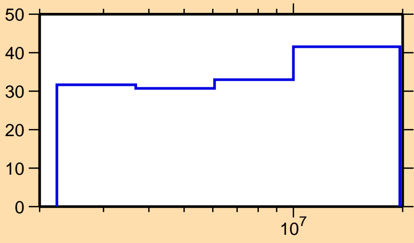
\Delta\sigma/\sigma vs. E for ^{99}\text{Mo}(n,\gamma)
