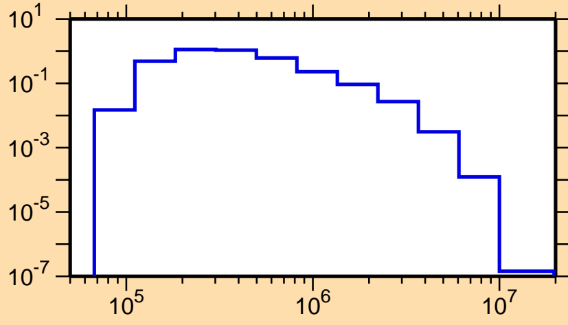
\sigma vs. E for ^{99}\text{Mo}(n,n_1)
