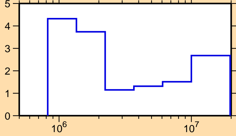
\Delta\sigma/\sigma vs. E for ^{99}\text{Mo}(n,\text{tot.})
