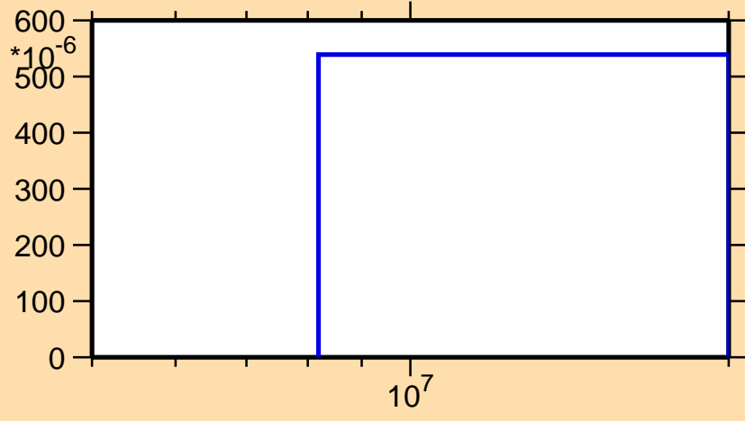
\sigma vs. E for ^{99}\text{Mo}(n,d)
