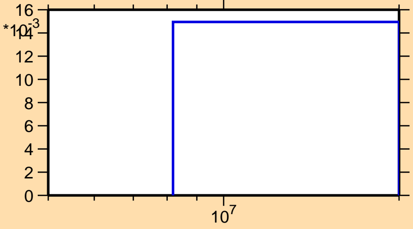
\sigma vs. E for ^{99}\text{Mo}(n,3n)
