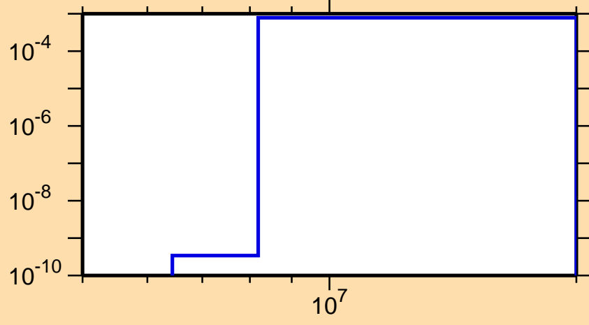
\sigma vs. E for ^{99}\text{Mo}(n,n\alpha)
