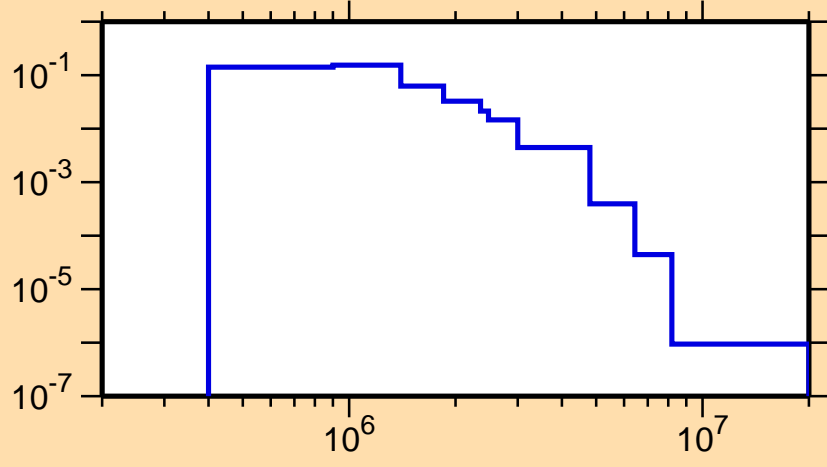
\sigma vs. E for ^{99}\text{Mo}(n,n_4)
