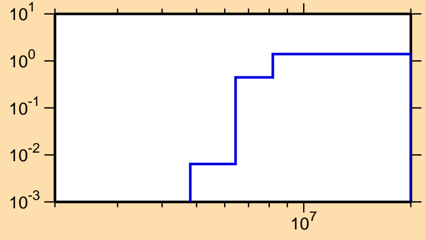
\sigma vs. E for ^{99}\text{Mo}(n,2n)
