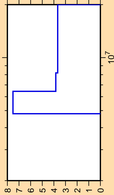
\Delta\sigma/\sigma vs. E for ^{99}\text{Mo}(n,2n)
