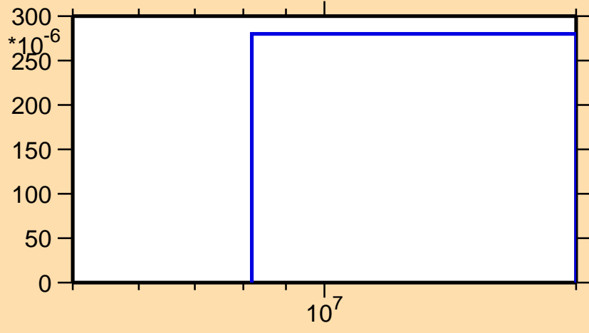
\sigma vs. E for ^{99}\text{Mo}(n,np)
