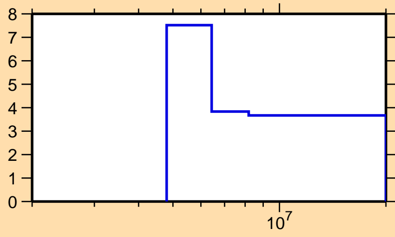
\Delta\sigma/\sigma vs. E for ^{99}\text{Mo}(n,2n)
