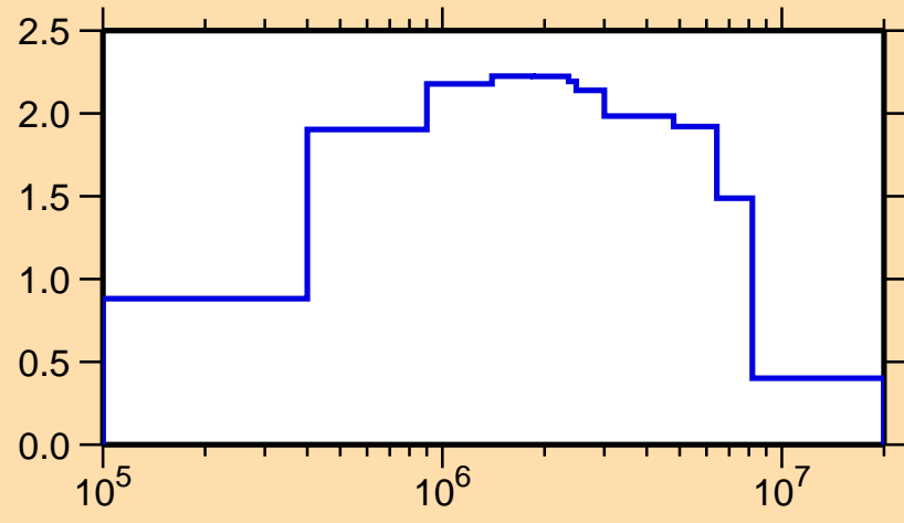
\sigma vs. E for ^{99}\text{Mo}(n,\text{inel.})
