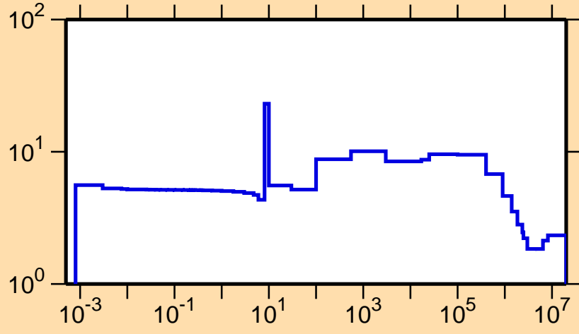
\sigma vs. E for ^{99}\text{Mo}(n,\text{el.})
