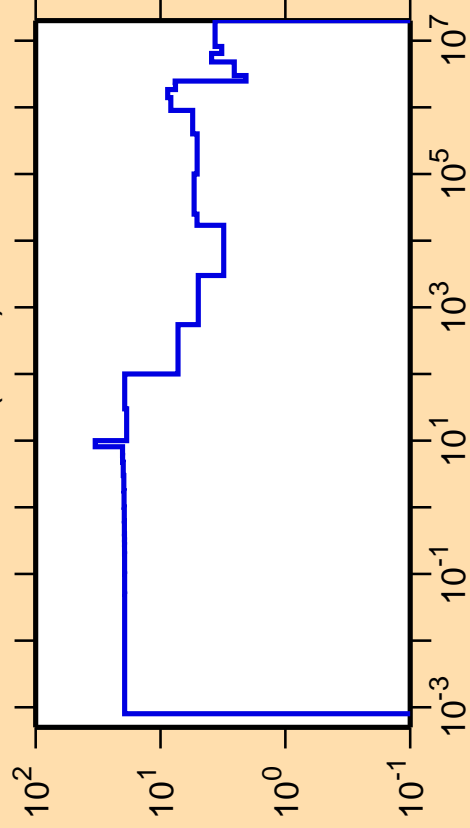
\Delta\sigma/\sigma vs. E for ^{99}\text{Mo}(n,\text{el.})
