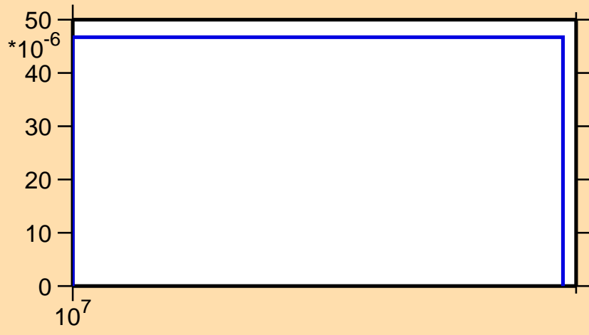
\sigma vs. E for ^{100}\text{Mo}(n,np)
