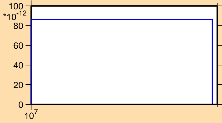
\sigma vs. E for ^{100}\text{Mo}(n,nd)
