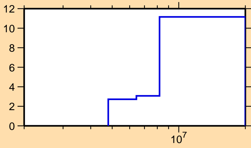
\Delta\sigma/\sigma vs. E for ^{100}\text{Mo}(n,n\text{cont.})
