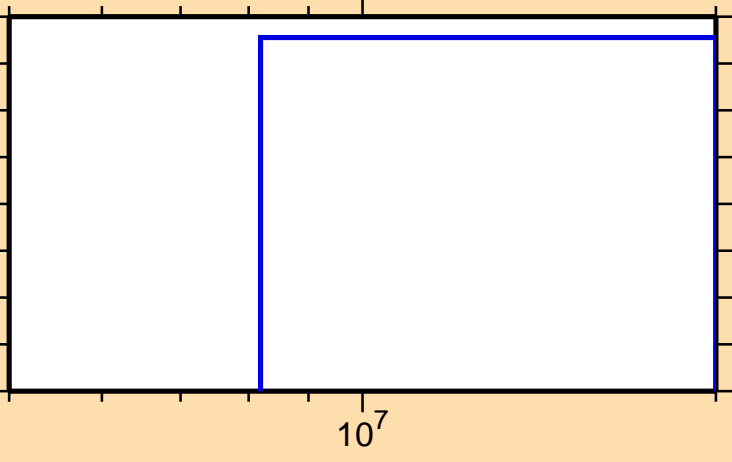
\sigma vs. E for ^{100}\text{Mo}(n,np)
