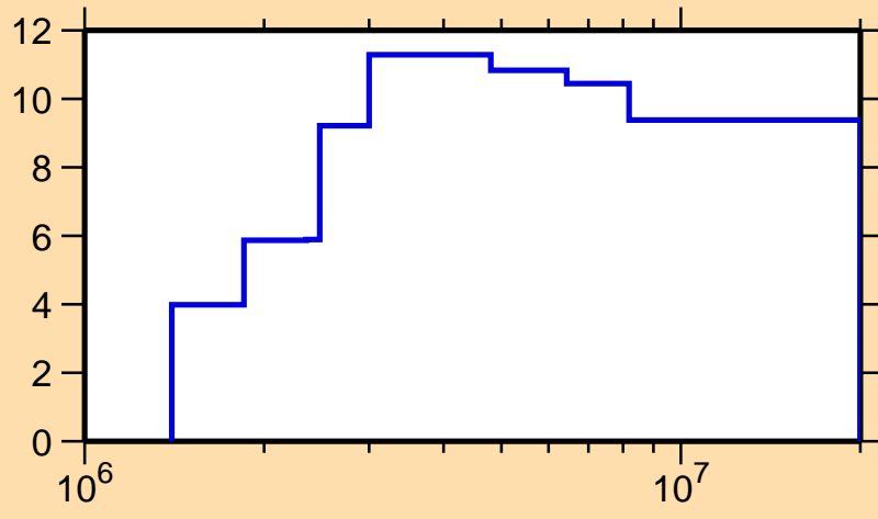
\Delta\sigma/\sigma vs. E for ^{100}\text{Mo}(n,n_1)
