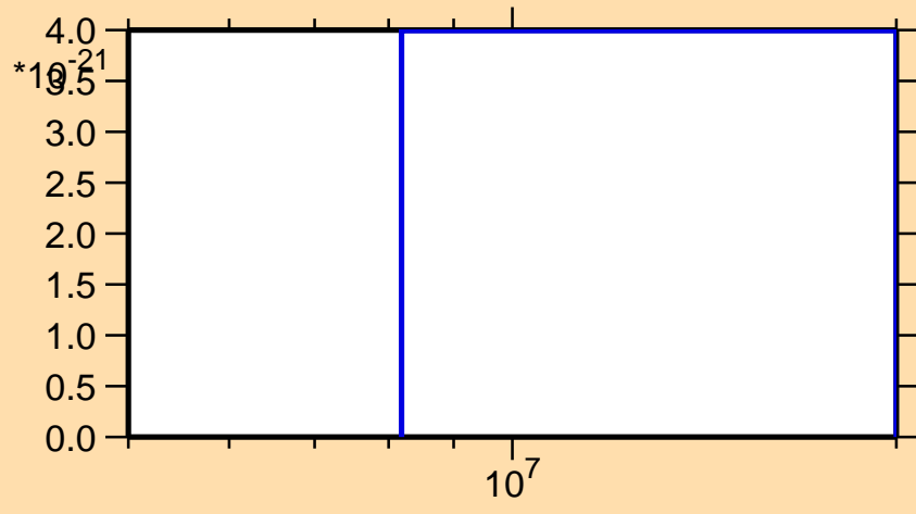
\sigma vs. E for ^{100}\text{Mo} (mt 34)
