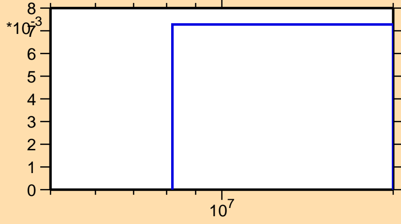
\sigma vs. E for ^{100}\text{Mo}(n,3n)
