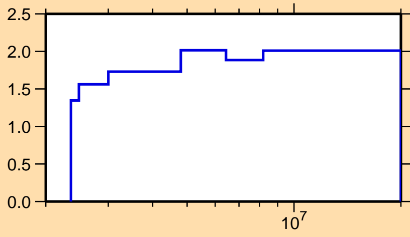
\Delta\sigma/\sigma vs. E for ^{100}\text{Mo}(n,n\text{onel.})
