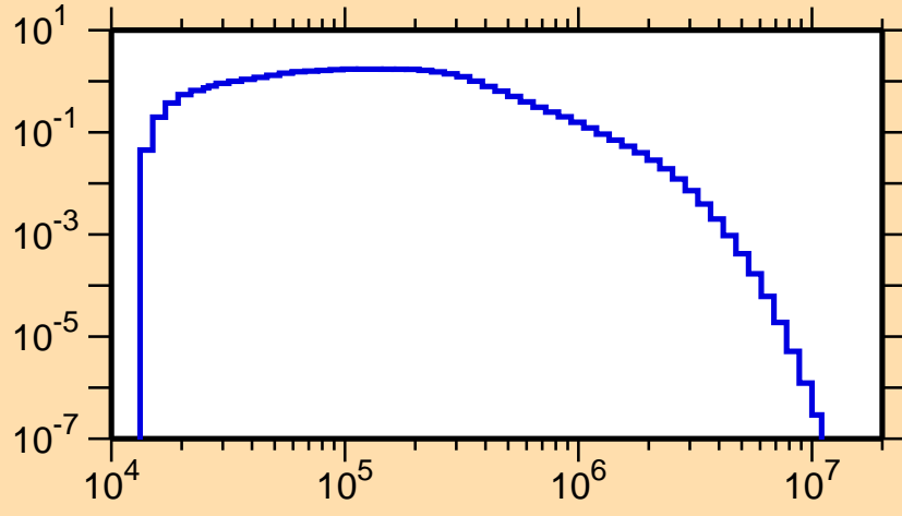
\sigma vs. E for ^{101}\text{Mo}(n,n_1)
