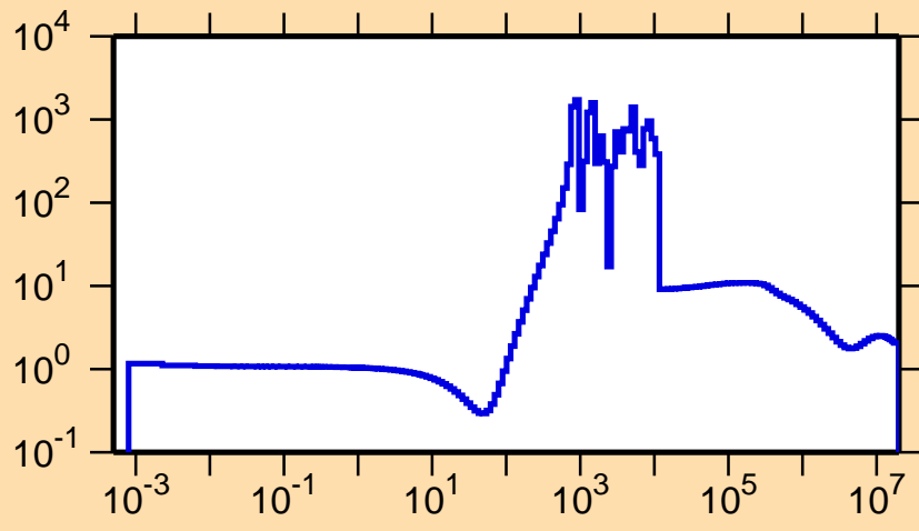
\sigma vs. E for ^{102}\text{Mo}(n,\text{el.})
