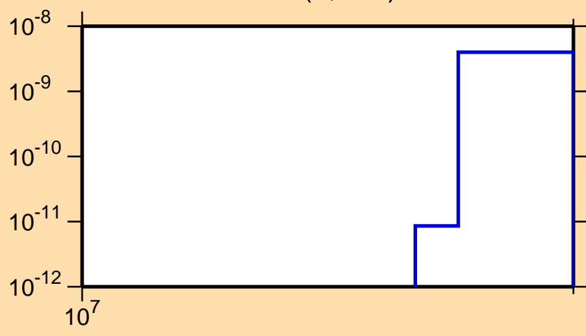
\sigma vs. E for ^{102}\text{Mo}(n,2n\alpha)
