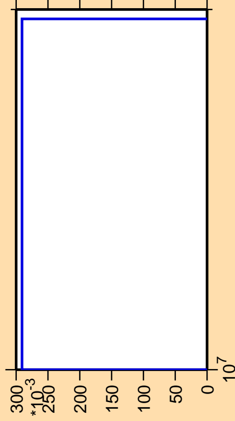
\Delta\sigma/\sigma vs. E for ^{102}\text{Mo}(n,\text{nd})
