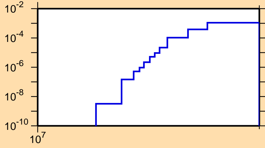
\sigma vs. E for ^{103}\text{Mo}(n,d)
