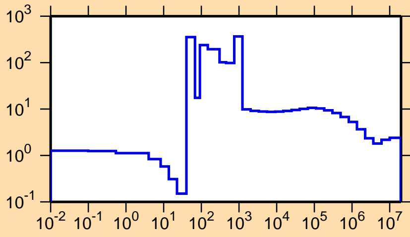
\sigma vs. E for ^{103}\text{Mo}(n,\text{el.})
