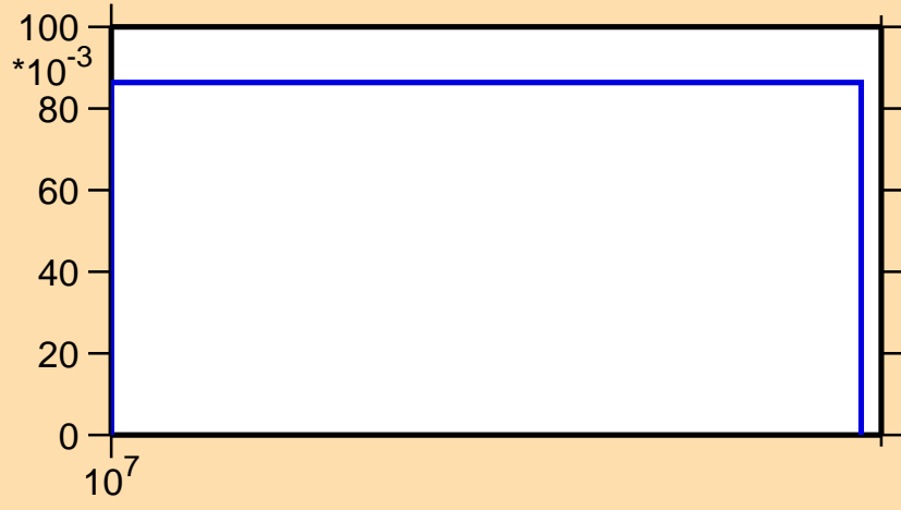
\sigma vs. E for ^{103}\text{Mo}(n,3n)
