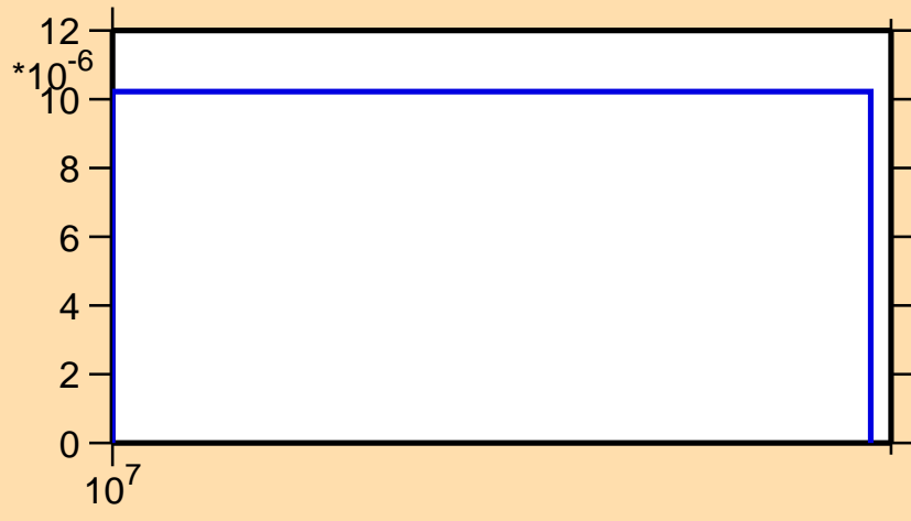
\sigma vs. E for ^{103}\text{Mo}(n,np)
