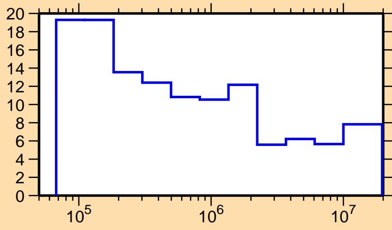
\Delta\sigma/\sigma vs. E for ^{103}\text{Mo}(n,\text{el.})
