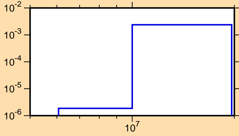
\sigma vs. E for ^{103}\text{Mo}(n,p)
