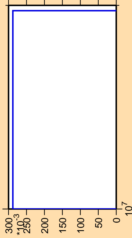
\Delta\sigma/\sigma vs. E for ^{103}\text{Mo}(n,2np)
