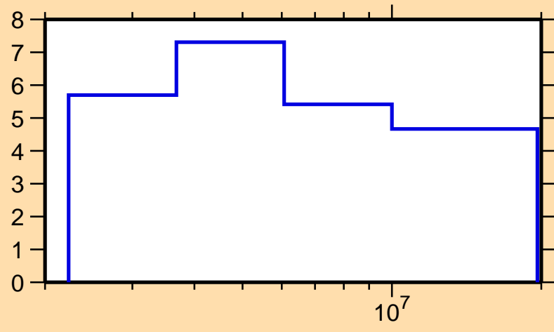
\Delta\sigma/\sigma vs. E for ^{103}\text{Mo}(n,\text{nonel.})
