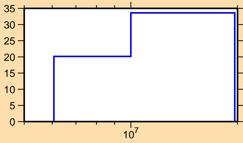
\Delta\sigma/\sigma vs. E for ^{103}\text{Mo}(n,n\text{cont.})
