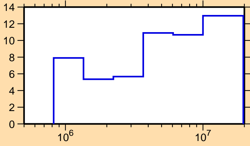
\Delta\sigma/\sigma vs. E for ^{103}\text{Mo}(n,\text{inel.})
