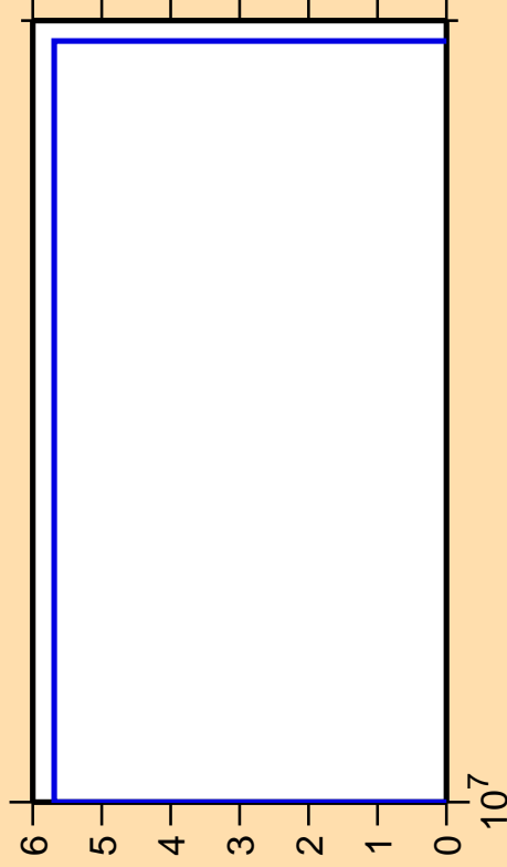
\Delta\sigma/\sigma vs. E for ^{103}\text{Mo}(n,nt)
