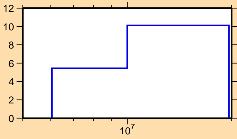
\Delta\sigma/\sigma vs. E for ^{103}\text{Mo}(n,2n)
