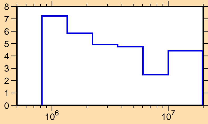
\Delta\sigma/\sigma vs. E for ^{103}\text{Mo}(n,\text{tot.})
