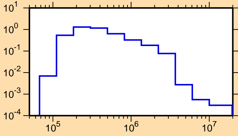
\sigma vs. E for ^{103}\text{Mo}(n,n_1)
