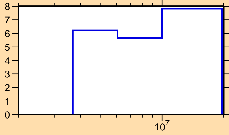
\Delta\sigma/\sigma vs. E for ^{103}\text{Mo}(n,\text{el.})
