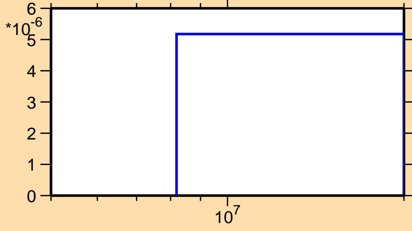
\sigma vs. E for ^{103}\text{Mo}(n,n\alpha)
