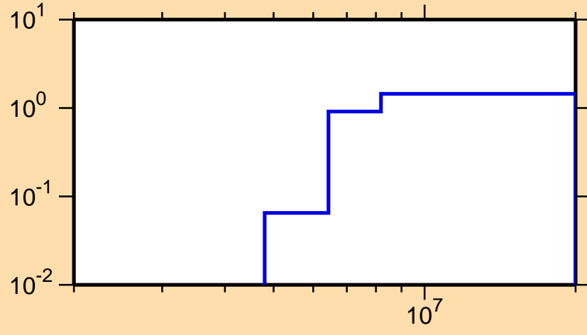
\sigma vs. E for ^{103}\text{Mo}(n,2n)
