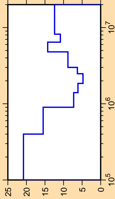
\Delta\sigma/\sigma vs. E for ^{103}\text{Mo}(n,\text{inel.})
