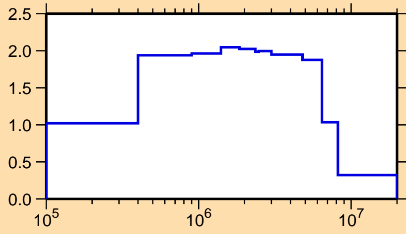
\sigma vs. E for ^{103}\text{Mo}(n,\text{inel.})
