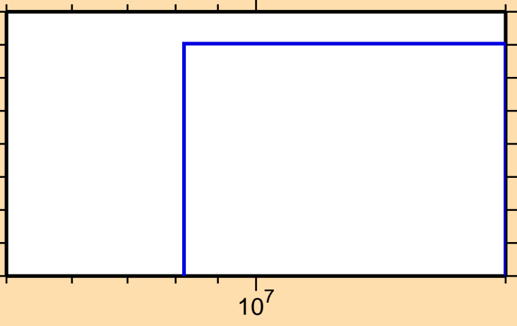
\sigma vs. E for ^{103}\text{Mo}(n,\text{nd})
