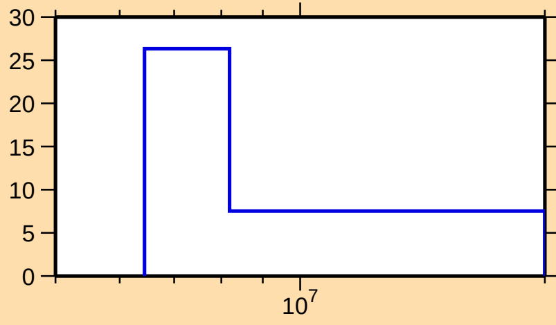
\Delta\sigma/\sigma vs. E for ^{104}\text{Mo}(n,2n)
