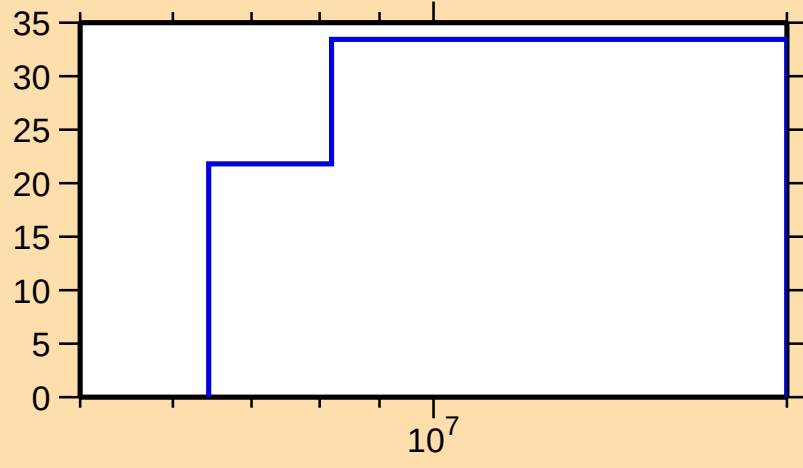
\Delta\sigma/\sigma vs. E for ^{104}\text{Mo}(n,\text{inel.})
