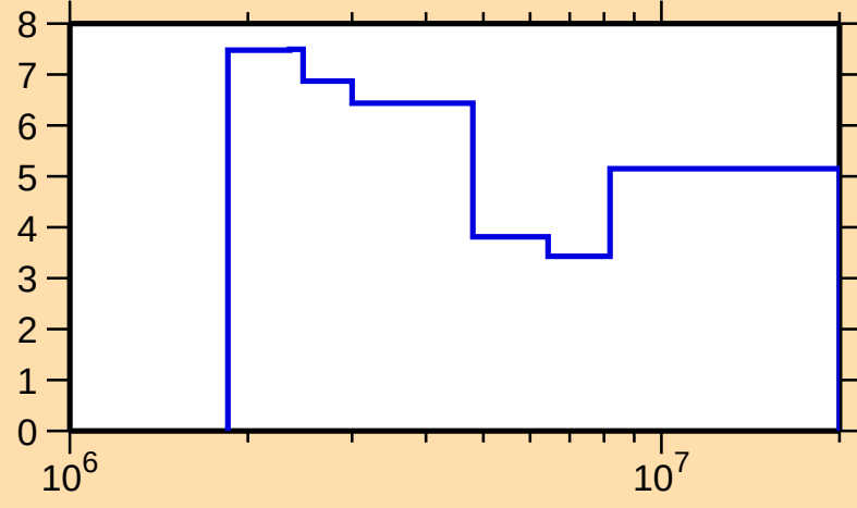
\Delta\sigma/\sigma vs. E for ^{104}\text{Mo}(\text{n},\text{tot.})
