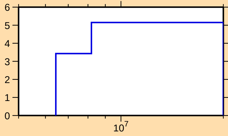
\Delta\sigma/\sigma vs. E for ^{104}\text{Mo}(n,\text{tot.})
