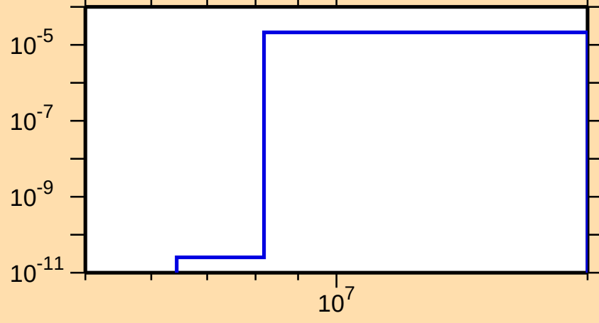
\sigma vs. E for ^{104}\text{Mo}(n,\alpha)
