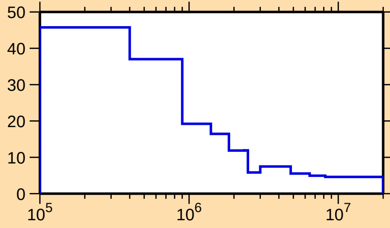
\Delta\sigma/\sigma vs. E for ^{104}\text{Mo}(\text{n,nonel.})
