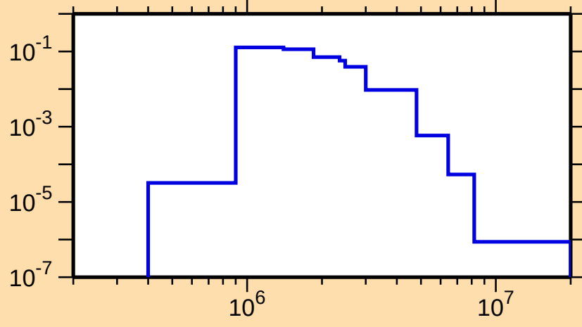
\sigma vs. E for ^{104}\text{Mo}(n,n_4)
