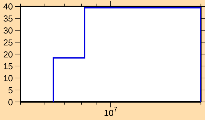
\Delta\sigma/\sigma vs. E for ^{104}\text{Mo}(n,n\text{cont.})
