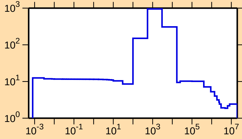
\sigma vs. E for ^{104}\text{Mo}(n,\text{el.})
