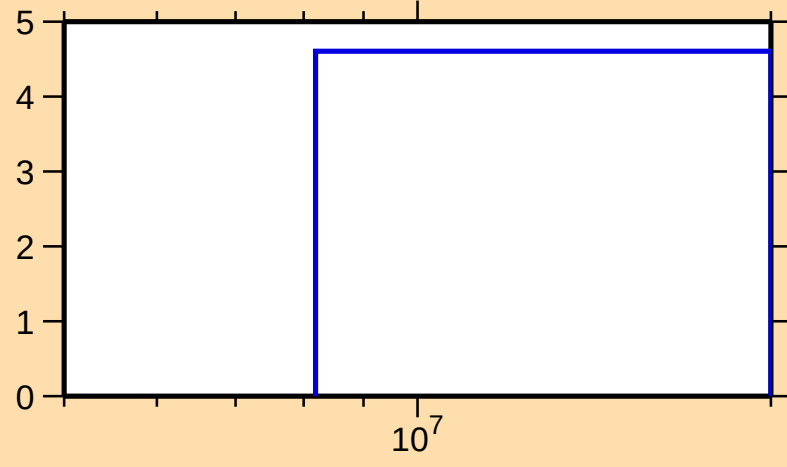
\Delta\sigma/\sigma vs. E for ^{104}\text{Mo}(n,\text{nonel.})
