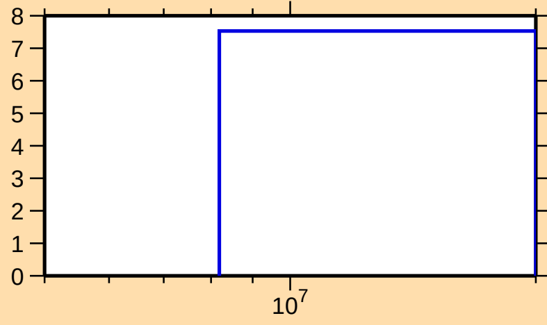
\Delta\sigma/\sigma vs. E for ^{104}\text{Mo}(n,2n)
