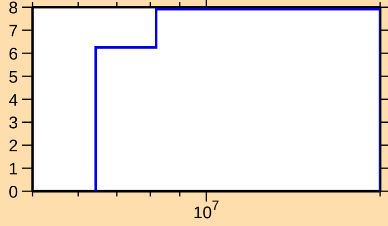
\Delta\sigma/\sigma vs. E for ^{104}\text{Mo}(n,\text{el.})
