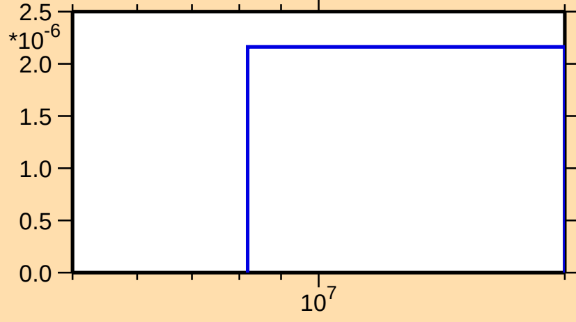
\sigma vs. E for ^{104}\text{Mo}(n,np)
