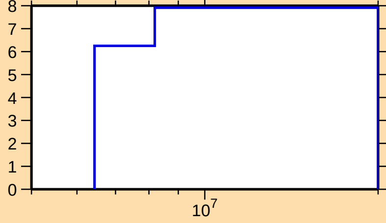
\Delta\sigma/\sigma vs. E for ^{104}\text{Mo}(n,\text{el.})
