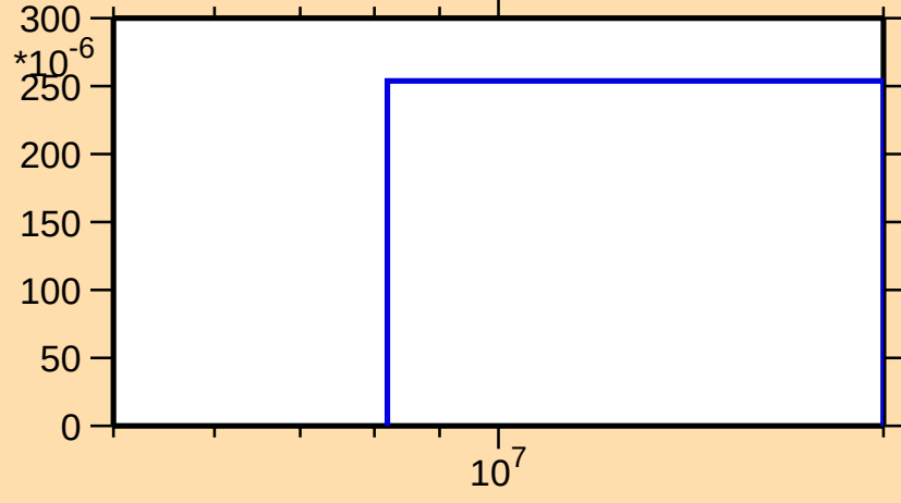
\sigma vs. E for ^{104}\text{Mo}(n,p)
