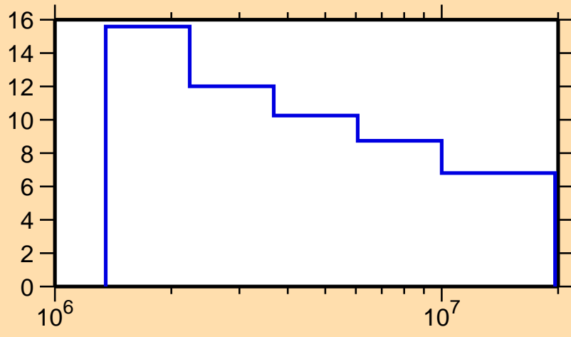
\Delta\sigma/\sigma vs. E for ^{105}\text{Mo}(n,n\text{onel.})
