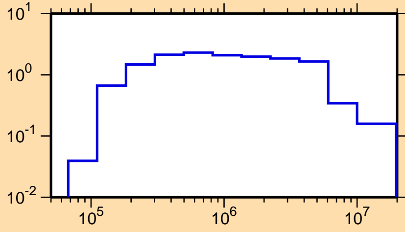
\sigma vs. E for ^{105}\text{Mo}(n,\text{inel.})
