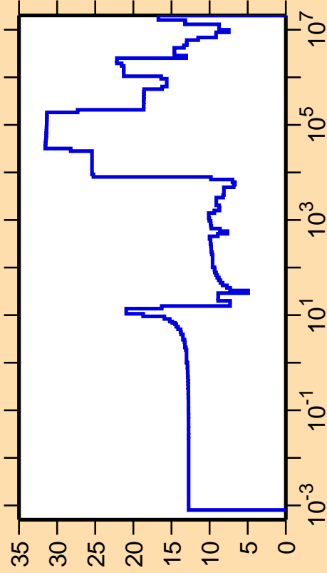
\Delta\sigma/\sigma vs. E for ^{106}\text{Mo}(n,\text{el.})
