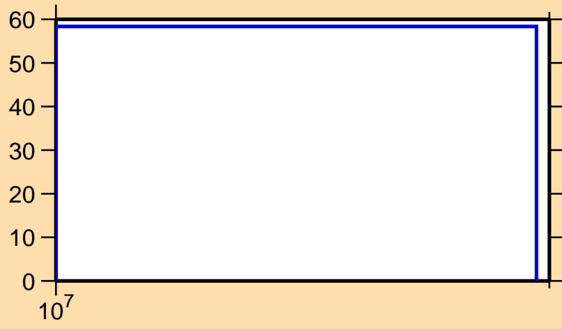
\Delta\sigma/\sigma vs. E for ^{106}\text{Mo}(n,n\text{cont.})
