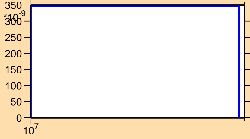
\sigma vs. E for ^{106}\text{Mo}(n,np)
