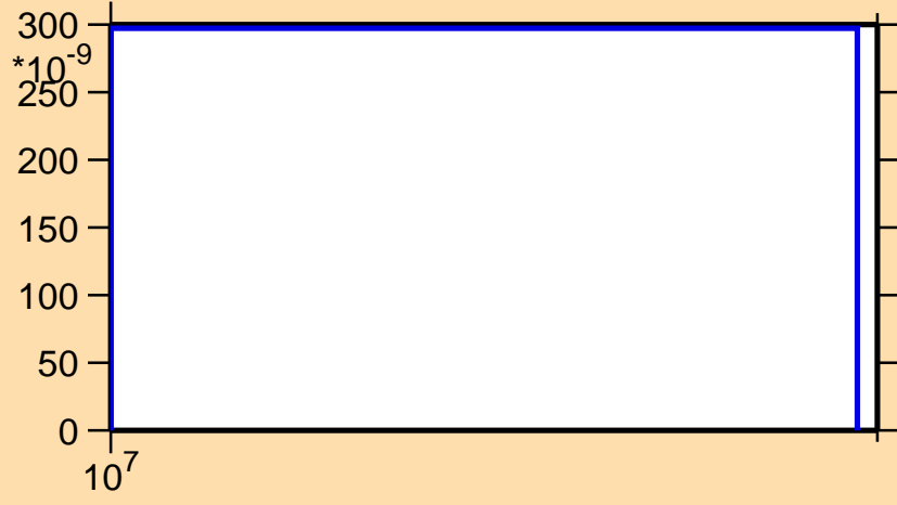
\sigma vs. E for ^{106}\text{Mo}(n,n\alpha)
