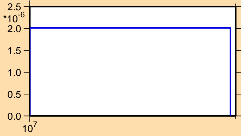
\sigma vs. E for ^{106}\text{Mo}(n,d)
