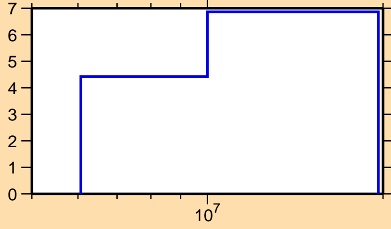
\Delta\sigma/\sigma vs. E for ^{106}\text{Mo}(n,\text{tot.})
