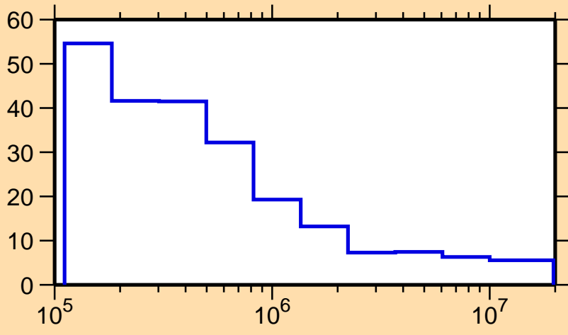
\Delta\sigma/\sigma vs. E for ^{106}\text{Mo}(n,\text{nonel.})
