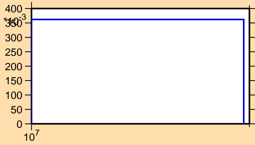
\sigma vs. E for ^{106}\text{Mo}(n,3n)
