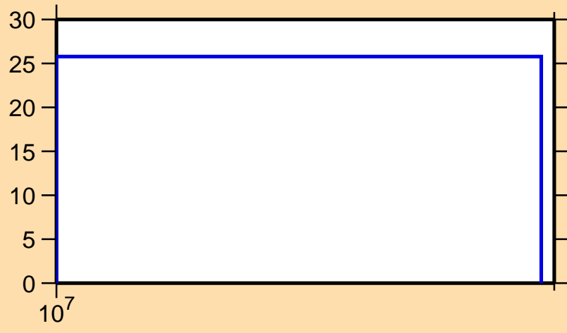
\Delta\sigma/\sigma vs. E for ^{106}\text{Mo}(n,2n)
