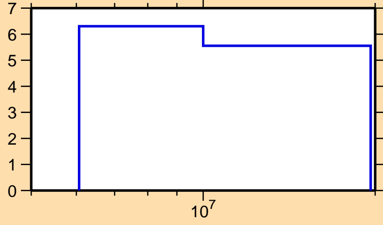
\Delta\sigma/\sigma vs. E for ^{106}\text{Mo}(n,\text{nonel.})
