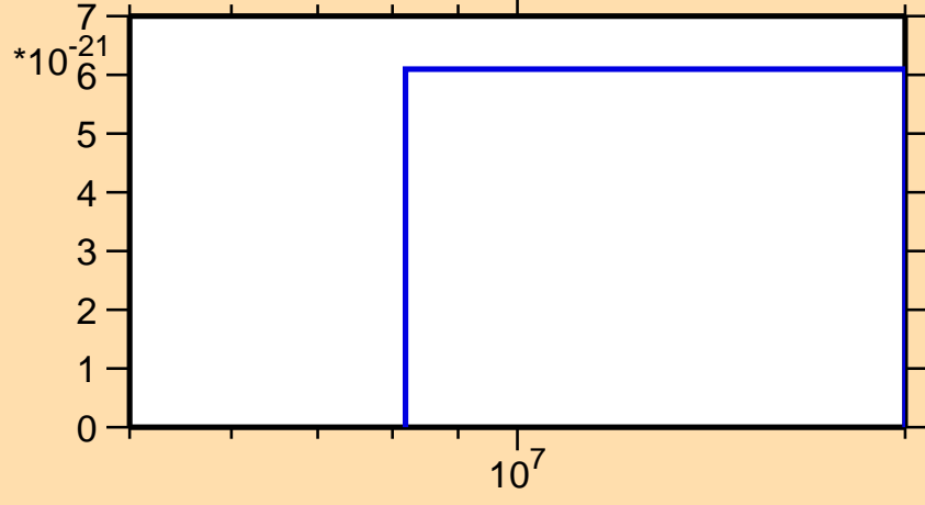
\sigma vs. E for ^{106}\text{Mo}(n,2np)
