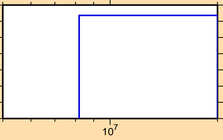
\sigma vs. E for ^{106}\text{Mo}(n,nt)
