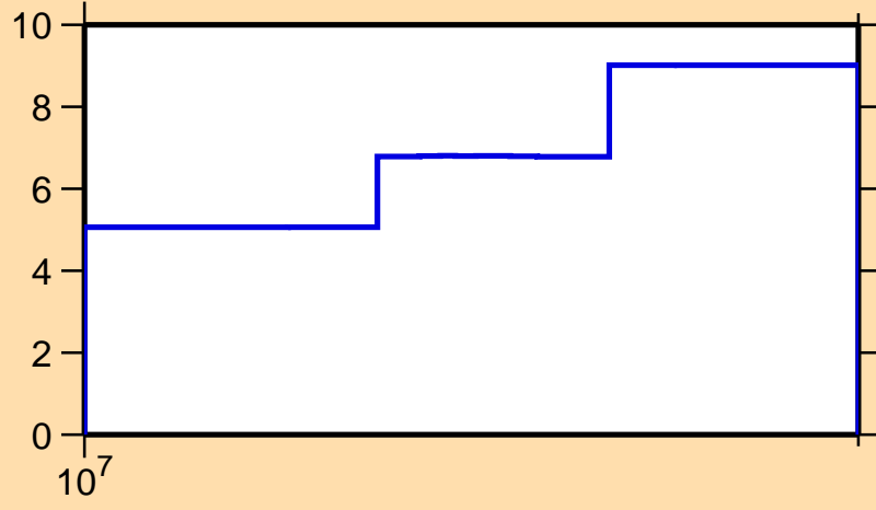
\Delta\sigma/\sigma vs. E for ^{108}\text{Mo}(n,el.)
