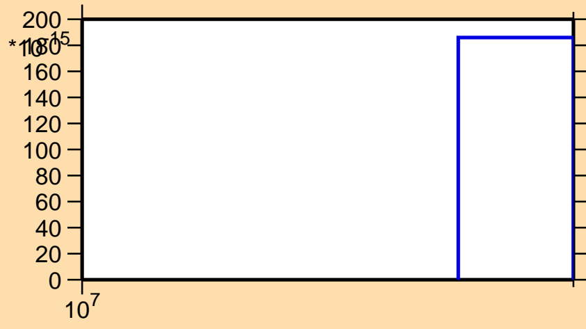
\sigma vs. E for ^{108}\text{Mo}(n,\text{nd})
