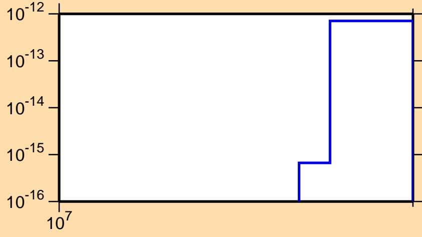
\sigma vs. E for ^{108}\text{Mo}(n,2n\alpha)
