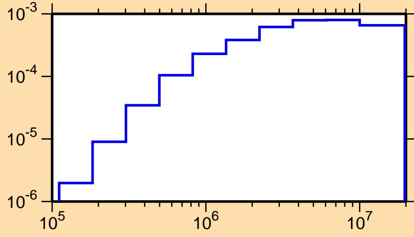
\sigma vs. E for ^{278}_{1}
