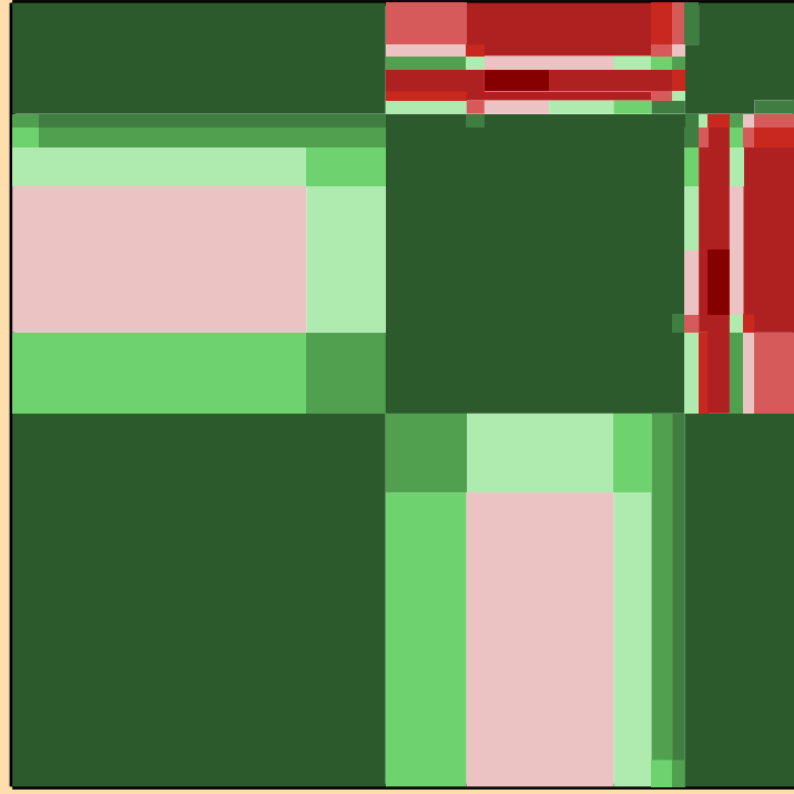
\sigma vs. E for ^{278}
